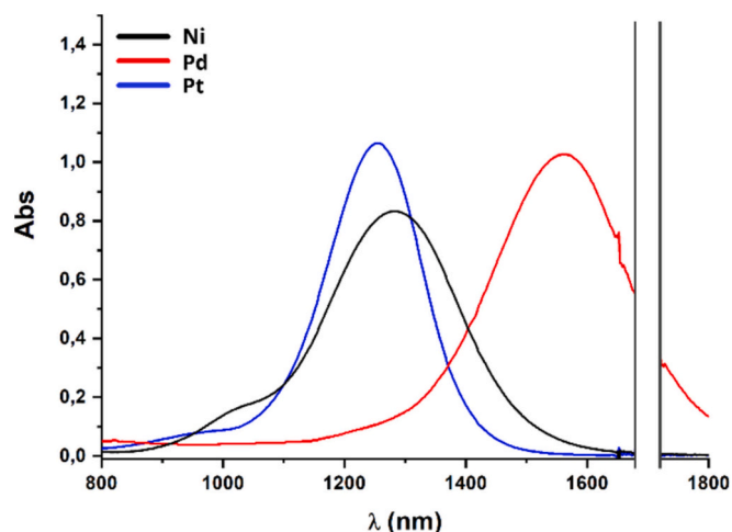
Fig. 3. NIR absorption spectra of [P][MEt]. M^{2+} = Ni^{2+}, Pd^{2+}, Pt^{2+} . The absorption between 1650 and 1750 nm was removed due to the presence of an artifact.
