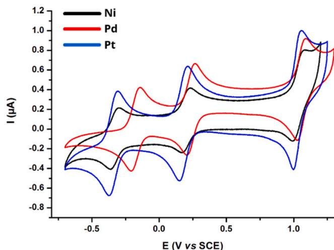
Fig. 2. Cyclic voltammograms of [P][MEt] M^{2+} = Ni^{2+}, Pd^{2+}, Pt^{2+} in CH_2Cl_2 with [NBu_4][PF_6] 0.1 M, E in V vs. SCE, scan rate of 100\text{ mV}\cdot\text{s}^{-1} .
