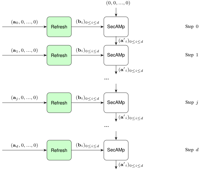
Fig. 6. Graphical Representation of \text{SecArithBoolModp} (The green (resp. white) gadgets will be proved d -SNI (resp. d -NI))
