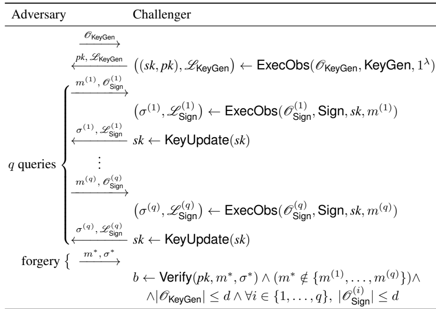
Fig. 2. d probing EUF-CMA game. \text{ExecObs} is a universal Turing machine that takes \mathcal{O}_{\text{alg}} as input and several other arguments, and returns the output of the algorithm on those arguments, together with \mathcal{L}_{\text{alg}} . Recall that the notation \mathcal{O}_{\text{alg}} corresponds to a set of the names of at most d intermediate values inside the algorithm alg. This set is chosen by attacker and the challenger provides \mathcal{L}_{\text{alg}} that is the leakage corresponding to each of the desired intermediate values.
