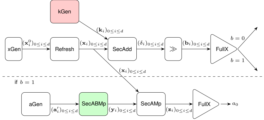
Fig. 5. Randomness Generation RG (The green (resp. white, red) gadgets will be proved d -SNI (resp. d -NI, unmasked))
