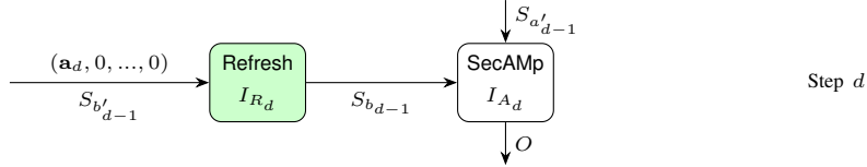
Fig. 7. Last step of SecArithBoolModp with probes (The green (resp. white) gadgets will be proved d -SNI (resp. d -NI))
