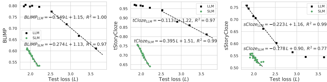
Figure 4: Correlation between downstream linguistic performance and test loss for LLMs and SLMs. Syntactic (BLIMP) and semantic (tStoryCloze and sStoryCloze) metrics are strongly linearly correlated with the upstream test loss before saturation.
