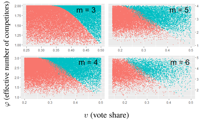
Figure 1: Effective seat thresholds for m = 3, 4, 5, 6 . Blue points indicate successful candidates, while red points – unsuccessful candidates.
