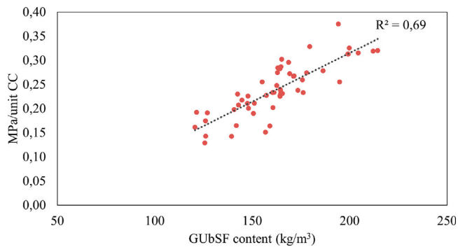
Fig. 11. Strength (MPa) provided by calced clay hydration based on GUBSF content.
