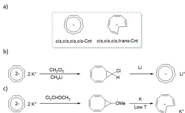
Fig. 1 (a) Isomers of the cyclononatetraenyl ligand, (b) original synthetic paths by Lalancette and Benson 27 and (c) synthetic path favoring the trans isomer. 28
