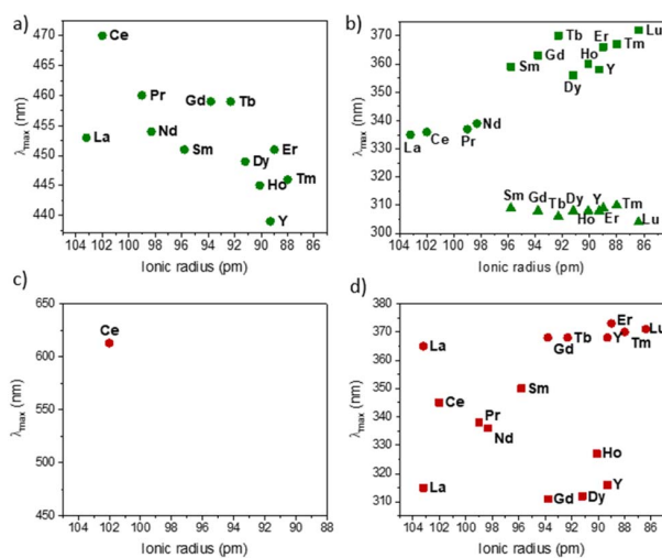
Fig. 8 Evolution of the maximum absorption of 2-Ln (the cis/trans ratio is given in Table 3) complexes wavelength around (a) 450 nm and (b) 300–370 nm and of 2-Ln- cis (made from the methodology proposed in literature 9,40 around (c) 400–650 nm and (d) 300–380 nm.
