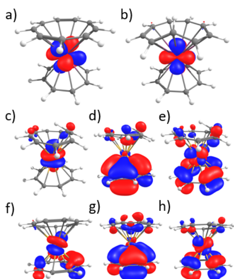
Fig. 9 Selected molecular orbitals (a) \alpha MO-HOMO-2 of 2-Ce- cis (SOMO). (b) \alpha MO-HOMO-2 of 2-Ce- trans (SOMO) (c) \alpha MO-HOMO-4 of 2-Sm- trans (d) \alpha MO-HOMO of 2-Sm- trans (e) \alpha MO-LUMO of 2-Sm- trans (f) \alpha MO-HOMO-8 of 2-Sm- cis (g) \alpha MO-HOMO of 2-Sm- cis (h) \alpha MO-LUMO of 2-Sm- cis .
