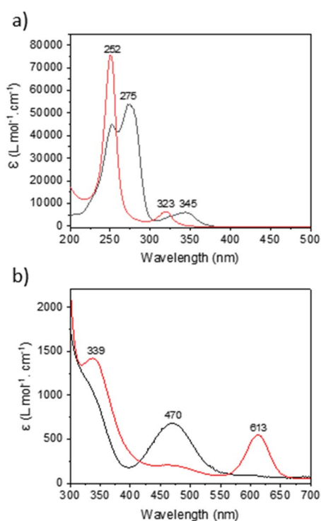
Fig. 7 UV-visible of (a) KCnt- trans (black) and KCnt- cis (red) and (b) trans (black) and cis (red) complexes of 2-Ce.
