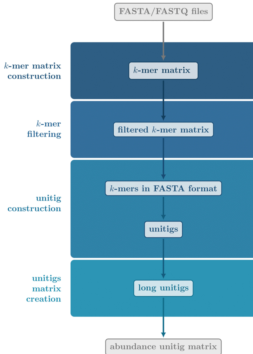
Figure 1. MUSET pipeline. It consists of four main steps: k -mer matrix construction, k -mer matrix filtering, unitig creation, and unitig matrix creation.
