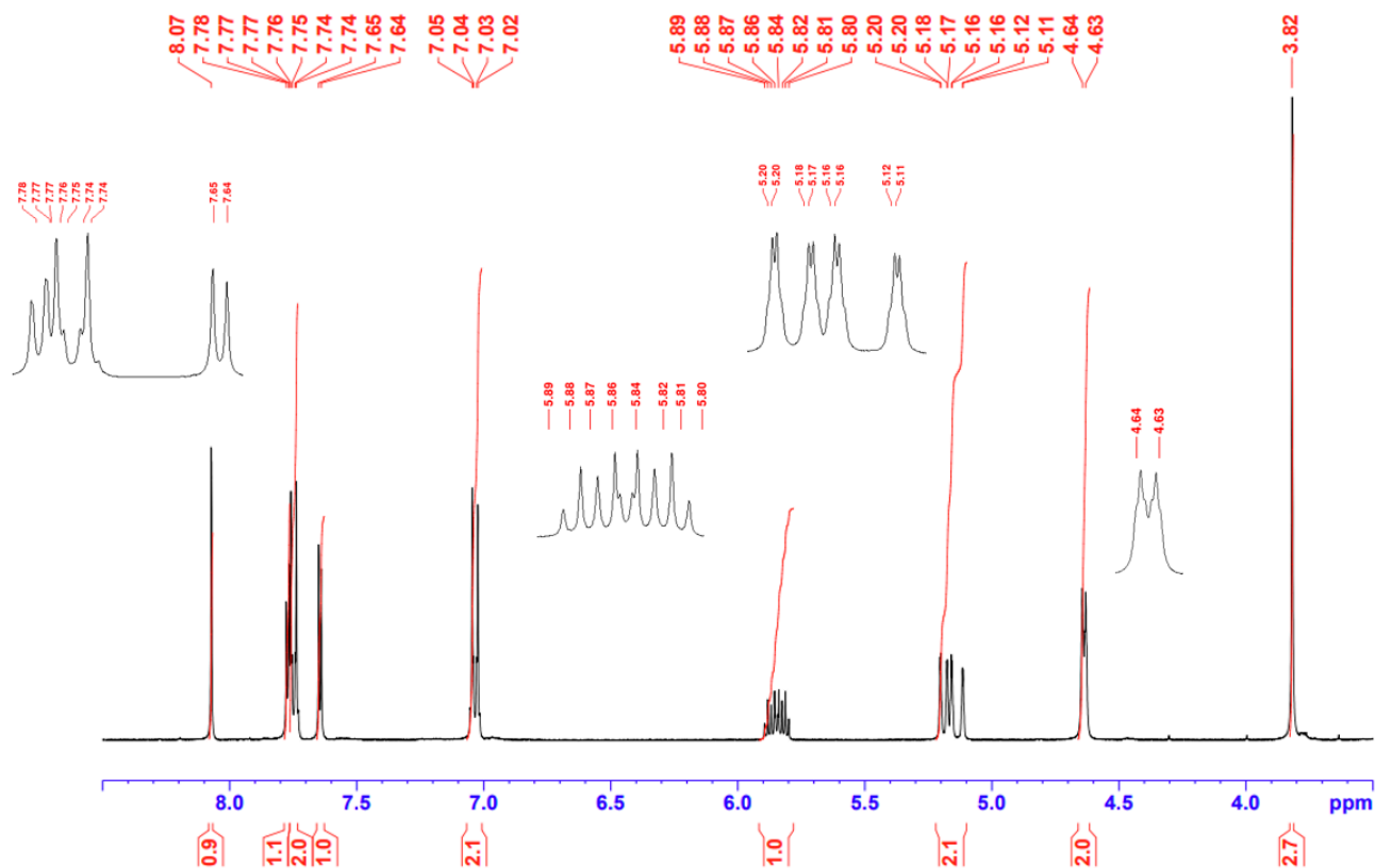
Figure 2. 1 H NMR spectrum (400 MHz, DMSO-d 6 ) of derivative 2.
