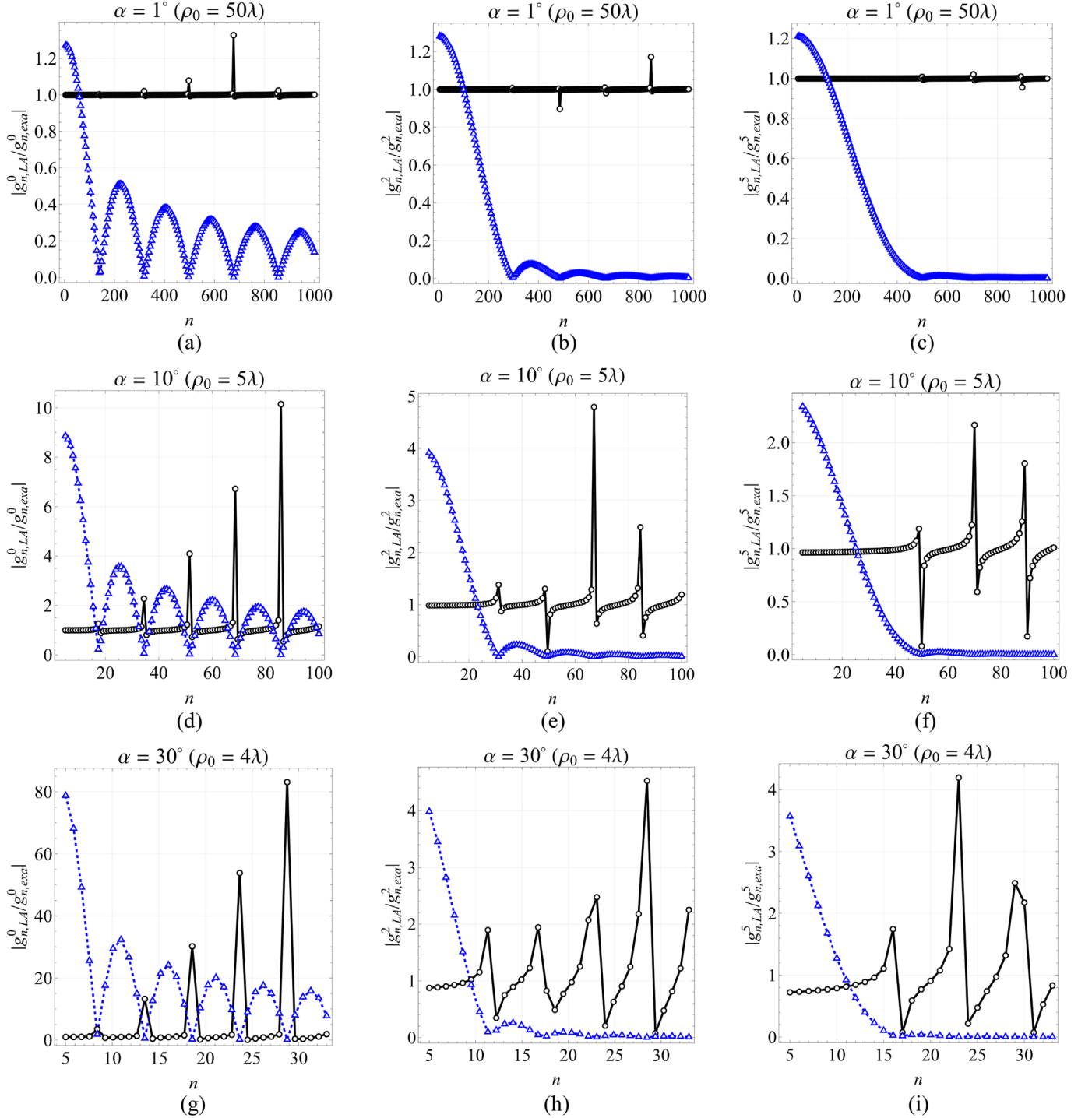
Figure 5. (a)–(c) Ratio |g_{n,LA}^m/g_{n,exa}^m| (black solid lines, with circular marks) for a Bessel beam with v = 0 for \alpha = 1^\circ and m = 0, 2 and 5 , respectively. (d)–(f) Same as before, now for \alpha = 10^\circ . (g)–(i) Same as (a)–(c), now for \alpha = 30^\circ . For reference purposes, the exact BSCs are also shown (blue dashed lines, with triangular marks), with multiplicative factors being introduced for better visualization. The choice of \rho_0 \neq 0 allows for non-zero BSCs for m \neq 0 but has not other implications in the comparison between the plots, since equation (39) does not depend on \rho_0 (had we chosen the same \rho_0 , the results would remain unchanged). The beam is assumed to be displaced along the x axis, that is, \phi_0 = 0 or, equivalently, \rho_0 = x_0 .
