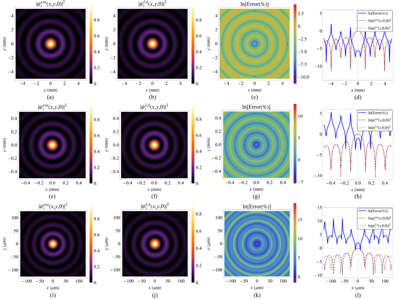
Figure 3. Exact and LA-remodeled field intensities |\psi_i^{exa}(x, y, 0)|^2 and |\psi_i^{LA}(x, y, 0)|^2 , and logarithmic percent errors \ln \left[ 100 \left| \frac{|\psi_i^{exa}(x, y, 0)|^2 - |\psi_i^{LA}(x, y, 0)|^2}{|\psi_i^{exa}(x, y, 0)|^2} \right| \right] for the zero-order Bessel beams of Figure 2 with \alpha = 1^\circ, 10^\circ and 50^\circ . (a)–(d) \alpha = 1^\circ . (e)–(h) \alpha = 10^\circ . (i)–(l) \alpha = 50^\circ . The corresponding BSCs are shown in Figure 2(a), (e) and (k), respectively.
