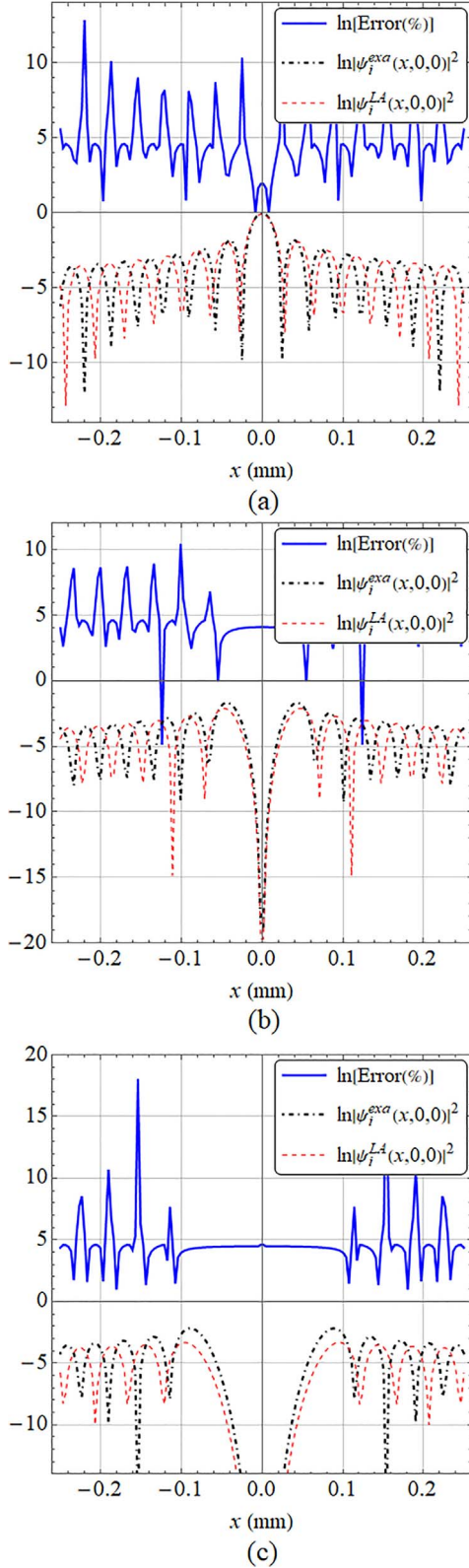
Figure 4. (a) Exact (black, dot-dashed) and LA-remodeled (red, dashed) field intensities |\psi_i^{ex\alpha}(x, 0, 0)|^2 and |\psi_i^{LA}(x, 0, 0)|^2 (in logarithmic scale), and logarithmic percent errors \ln \left[ 100 \frac{(|\psi_i^{ex\alpha}(x, 0, 0)|^2 - |\psi_i^{LA}(x, 0, 0)|^2)|}{|\psi_i^{ex\alpha}(x, 0, 0)|^2} \right] for an on-axis Bessel beams with \alpha = 50^\circ , for v = 0 . (b) and (c) Same as (a), but now for v = 3 and 7 , respectively.
