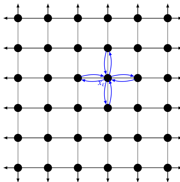
Figure 1. Our refining spatial grid D_\varepsilon in dimension d = 2 , with periodic boundary conditions. The arrows are drawn to indicate that opposite edges are identified. The arrows at the bottom correspond to the arrows at the top, and those on the left correspond to those on the right. \varepsilon is the mesh size of the grid. The blue arrows around site x_\varepsilon indicate the possible movements of individuals from and to x_\varepsilon .
