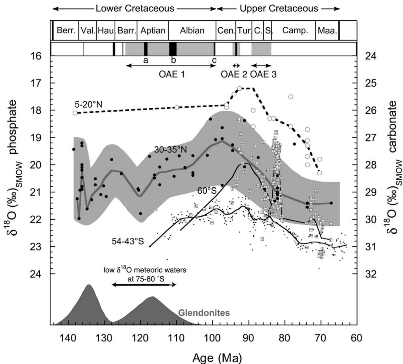
Figure 2. Comparison of \delta^{18}\text{O} variations between fish remains (open circles: Kolodny and Raab [1988], bones, teeth, and vertebra; and solid circles: this work, teeth), planktonic foraminifera (crossed squares: Huber et al. [1995]), and fine fraction and bulk carbonates (dots: Clarke and Jenkyns [1999]). Absolute ages are derived from the timescale of Gradstein et al. [1994]. The curves for oxygen isotope data are based on the locally weighted least squared error method using a smoothing coefficient of 20%. Based on fractionation equations, two isotopic scales are given to facilitate the comparison of \delta^{18}\text{O} values of both carbonates and phosphates [Epstein et al. , 1953; Longinelli and Nuti, 1973; Kolodny et al. , 1983]. Paleolatitudes are estimated from the maps proposed by Scotese et al. [1988]. Glendonite events, indicated with an arbitrary scale, are from Price [1994]. Oceanic anoxic events, OAE, are from Breheret [1994], Crumière et al. [1990], Baudin et al. [1999], and Reboulet et al. [2000] for the southeast of France (black rectangles) and from Jenkyns [1980] for worldwide OAE (gray rectangles). Note that the gray rectangles represent time intervals including the cumulative occurrence of OAEs around the globe. Low- \delta^{18}\text{O} meteoric waters at 75–80°S within the lower Cretaceous are from Gregory et al. [1989]. See Figure 1 for other abbreviations.
