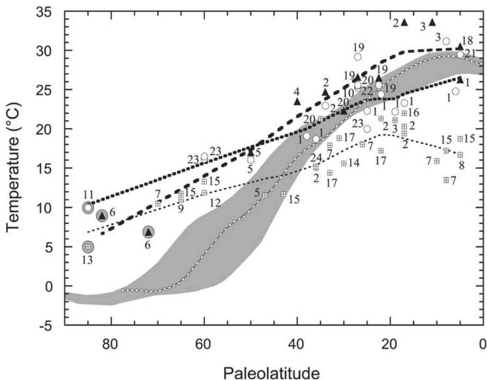
Figure 3. Sea surface latitudinal temperature gradients. Open squares: present day; open circles: Albian-Cenomanian; solid triangles: Turonian, and crossed squares: Maastrichtian. The present-day annual sea surface temperature gradient has been established using the data library LEVITUS94 for the south Pacific Ocean. The gray envelope marks the extension of the modern gradient, if including North Pacific, South Atlantic, and North Atlantic surface temperatures. Sources for the Cretaceous gradients are: 1. Sellwood et al. [1994], 2. This work, 3. Kolodny and Raab [1988], 4. Jenkyns et al. [1994], 5. Clarke and Jenkyns [1999], 6. Herman and Spicer [1996], 7. D'Hondt and Arthur [1996], 8. Li and Keller [1999], 9. Stott and Kennett [1990], 10. Norris and Wilson [1998], 11. Spicer and Parrish [1986], 12. Pirrie and Marshall [1990], 13. Parrish and Spicer [1988], 14. Saito and Van Donk [1974], 15. Barrera et al. [1997], 16. Lécuyer et al. [1993], 17. Frank and Arthur [1999]. 18. Wilson et al. [2002], 19. Stoll and Schrag [2000], 20. Huber et al. [2002], 21. Norris et al. [2002], 22. Wilson and Norris [2001], 23. Fassell and Bralower [1999], 24. Li and Keller [1998]. The temperatures have been averaged when several data were available for the different time slices. Isotopic temperatures for planktonic foraminifera are calculated from the published \delta^{18}\text{O} values by using the equation of Erez and Luz [1983]. For bulk carbonates and fish remains, temperatures were calculated using equations given by Anderson and Arthur [1983], and Kolodny et al. [1983], respectively, using a \delta^{18}\text{O}_{\text{seawater}} of -1\text{‰} SMOW. For sources 6, 11, and 13, temperature estimates (mean annual temperature) are provided by paleobotanical studies, mainly from leaf physiognomy, and are distinguished from the rest of the data by a gray shaped circle.
