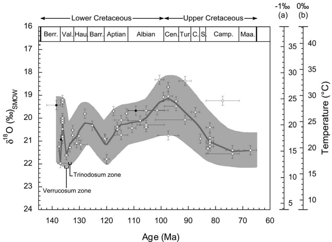
Figure 1. Evolution of \delta^{18}\text{O} values of fish teeth from the western Tethys during the Cretaceous (Table 1). Open circles mark samples with a La/Sm ratio higher than 0.3 and solid circles mark samples with a La/Sm ratio lower than 0.3 (see the text for more details). Isotopic temperatures are calculated using the equation of Kolodny et al. [1983] with \delta^{18}\text{O}_{\text{seawater}} of (a) -1\text{‰} and (b) 0\text{‰} . Absolute ages are derived from the timescale of Gradstein et al. [1994]. The solid curve represents the variation of the mean value with time, computed using a fitting function based on the locally weighted least squared error method with a smoothing factor of 20%, and its envelope at \pm 1\text{‰} . The position of the sample on its temporal error bar is determined by its most probable stratigraphic position. Two important ammonite zones are given for reference. Abbreviations are: Berr = Berriasian; Val = Valanginian; Hau = Hauterivian; Barr = Barremian; Cen = Cenomanian; Tur = Turonian; C = Coniacian; S = Santonian; Camp = Campanian; Maa = Maastrichtian.
