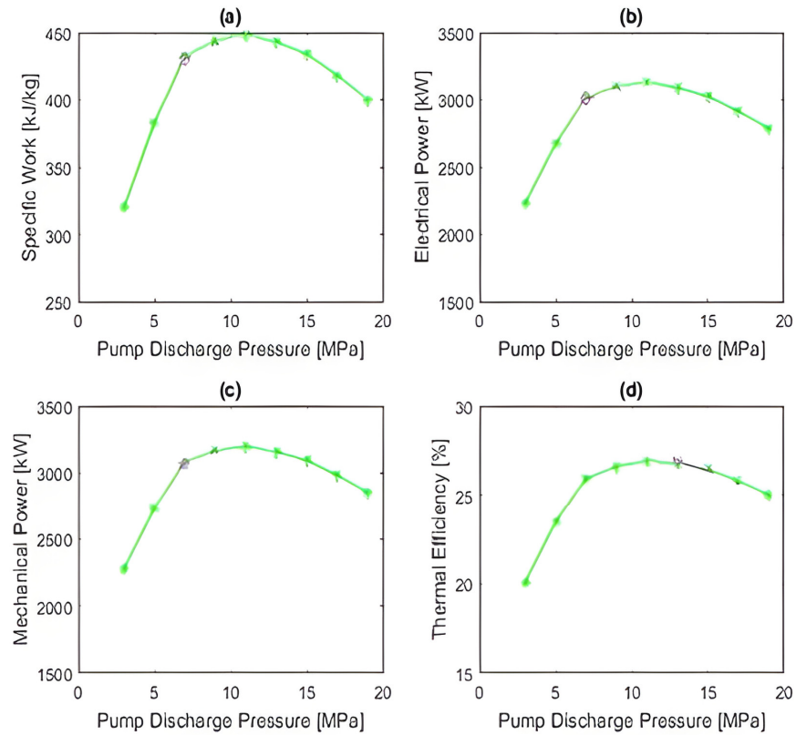
Figure 9. Influence of pump discharge pressure on performance parameters.
