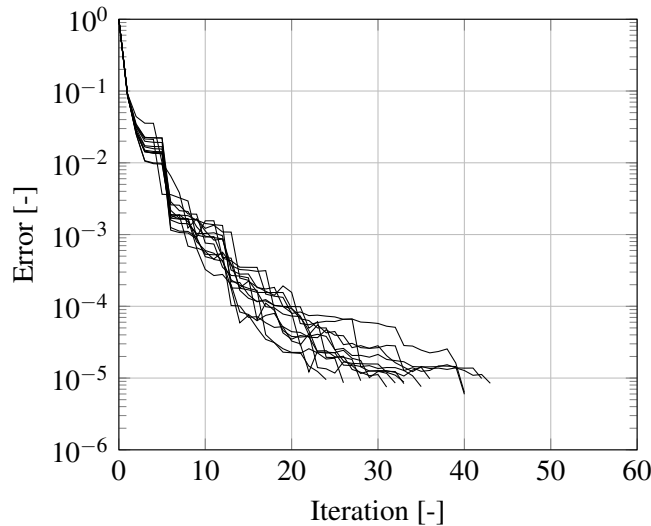
FIGURE 3 – PGD error during each simulations presented in this work.
