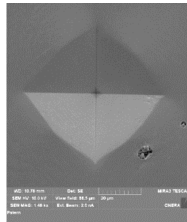
FIGURE 7. Typical imprint of a Vickers test on Ni-based superalloy under a load of 10 N.
