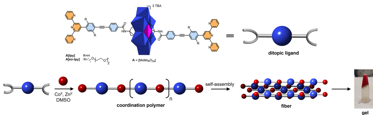
Figure 1. Molecular structures of the organic and hybrid compounds and schematic representation of the coordination-driven gelation process (TBA: tetrabutylammonium).
