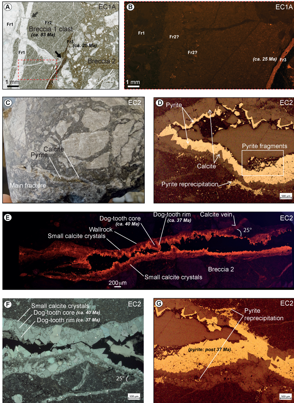
Figure 3. Microphotographs of thin sections from samples of the La Rouvière Fault Core. (A) Scan of the sample EC1A entire thin section showing the crosscutting relationships between fracture families and breccia phases. The left part of the image is a clast from breccia 1, (B) Close-up CL image showing the highly bright orange luminescence of Fr3 and crosscutting relationships with previous fractures and breccias, (C) EC2 sample showing main sigmoidal shape fracture filled by calcite and pyrite crystals at the scale of the hand specimen, (D) EC2 fracture filled with calcite and pyrite observed in reflected light. Note the pyrite crystals fragmentation at the bottom right, (E) Main EC2 fracture in cathodoluminescence image (CL), (F) Calcite growing episodes of main EC2 vein under cross polarized light, (G) Main and second phase of pyrite crystallization in reflected light. Note that U–Pb ages obtained in this study have been added on photographs for clarity.
