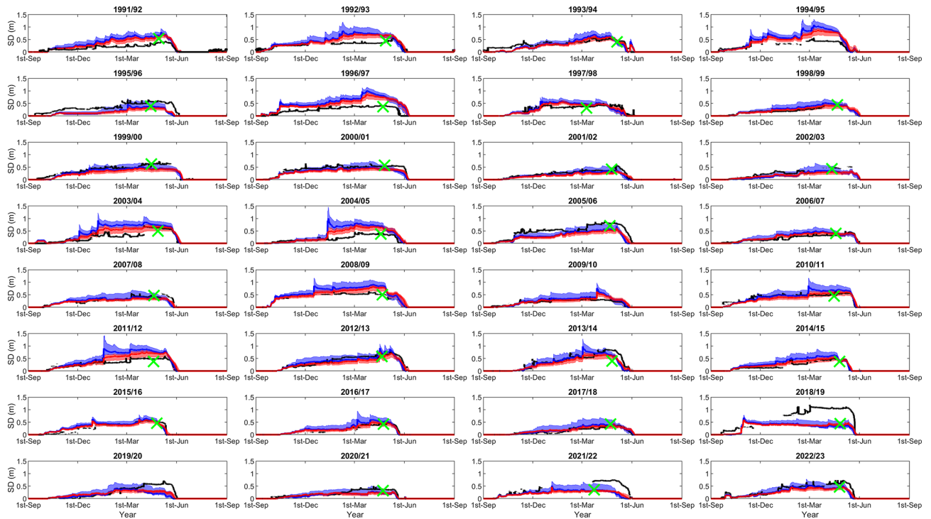
Figure B2. Time series of hourly simulated snow depth (m) at TVC for the 1991–2023 snow seasons. Maximum and minimum values of the default (blue) and Arctic (red) SWS2-Crocus ensembles are represented by the shaded regions. Median values of both ensembles are represented by solid-coloured lines. SR50 measurements are displayed using solid black lines, and snow course measurements are green crosses.
