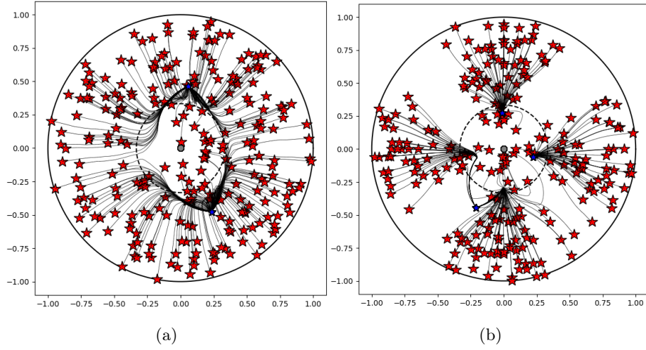
Fig. 4: Comparison of different entrance laws over the full circle. On the left (a), the entrance law (\theta_{\text{in}}, \rho_{\text{in}}) is uniform over the whole ball. We clearly observe two phases of the process: during the first phase is only the radii evolve. Once the agents' self-confidence get closer to the PRE value, here \rho^\star = \frac{1}{3} , the radius dynamics decelerates and the angular dynamics expands, namely due to fluctuations, also called 'finite-type' effect.
