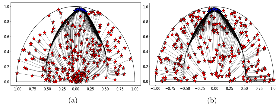
Fig. 3: Comparison of different entrance laws. On the left (a), we took as entrance law uniform in the opinion, that is \theta_{\text{in}} = \text{Unif}[0, \pi] , but with concentration on the center by choosing \rho_{\text{in}} = \text{Unif}[0, 1] . And on the right (b), we took as entrance law the uniform spatial measure: (\theta_{\text{in}}, \rho_{\text{in}}) = \text{Unif}(\mathbb{B}_+) .
