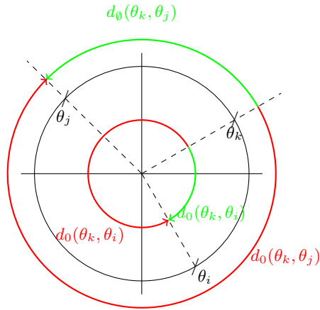
Fig. 2: A simple scheme to explain the computation of angle subtraction and distance in the circle. Here, we have three angles \theta_k = \frac{\pi}{3} , \theta_j = \frac{3\pi}{4} and \theta_i = \frac{5\pi}{3} . The arc (\theta_j -_{\mathbb{C}} \theta_k) is positive, flowing in the trigonometric direction. On the contrary, the arc (\theta_i -_{\mathbb{C}} \theta_k) is negative: in order to reach \theta_i starting from \theta_k , one shall run along the circle toward the anti-trigonometric direction.
