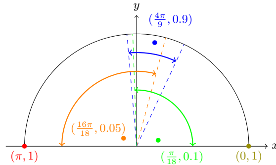
Fig. 1: A simple scheme to explain dynamics (1) with 5 agents and their respective radius of influence.
