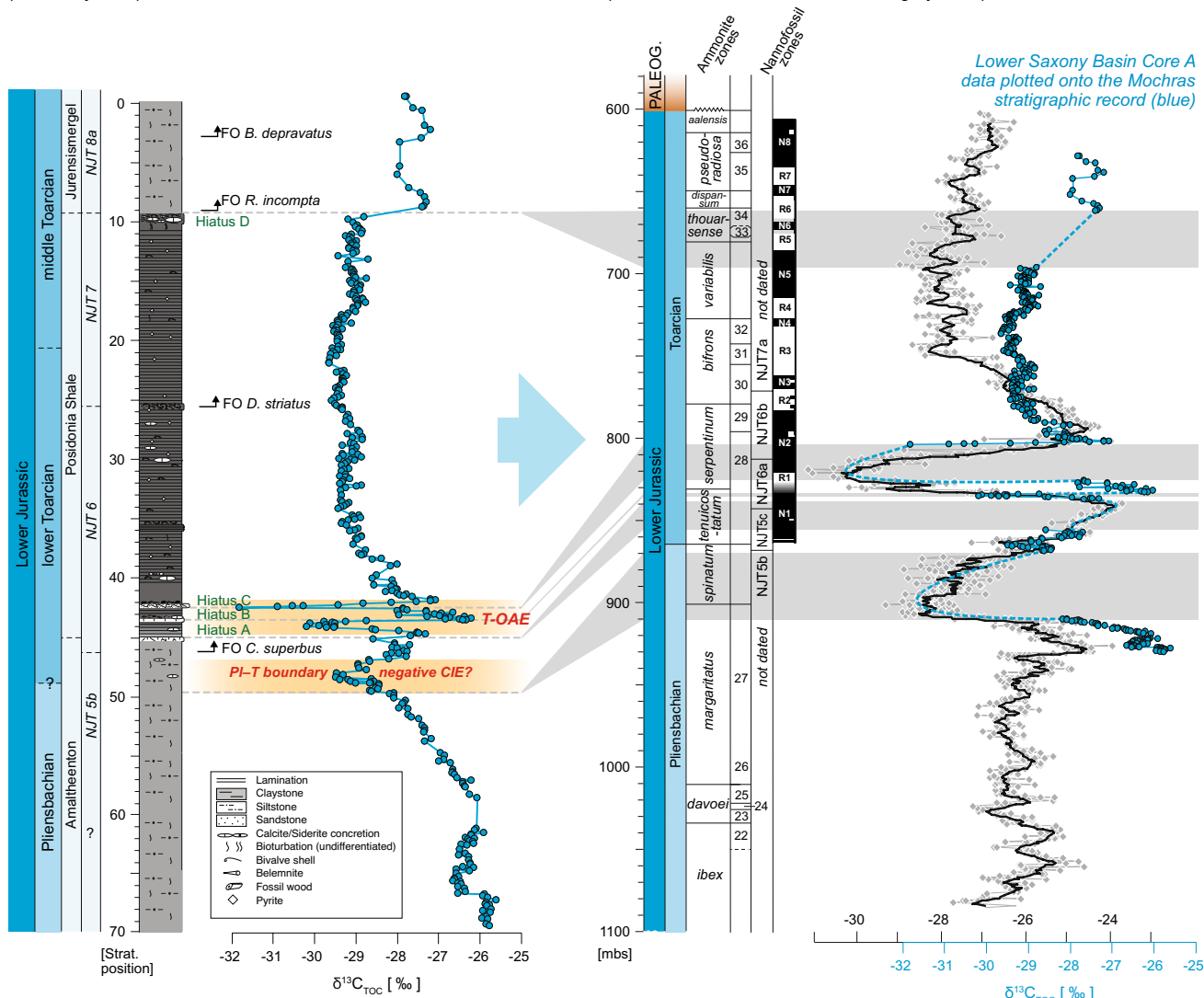
Fig. 7 Integrated stratigraphic record for Core A, with the \delta^{13}C_{TOC} record from Core A, superimposed on the stratigraphic record of the Mochras core. Ammonite zonation from Ivimey-Cook (1971), Page
