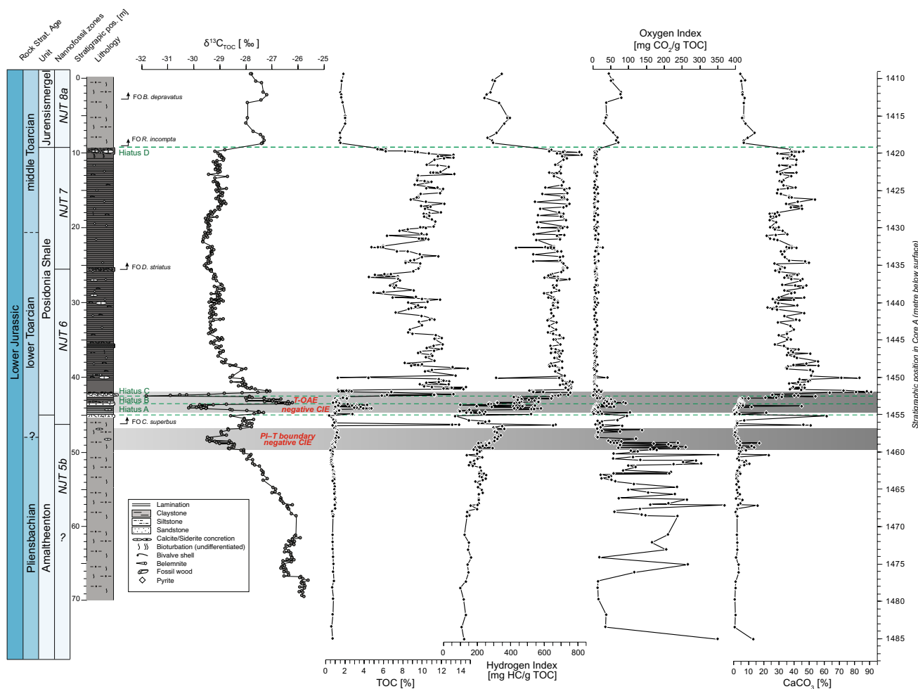
Fig. 4 Lithological log of Core A with First Occurrences of calcareous nannofossils, stratigraphic location of main hiatus horizons, and the generated \delta^{13}C_{TOC} (this study), Total Organic Carbon (TOC: this study, Hooker et al. 2020; Dickson et al. 2022), Hydrogen Index (HI: this study), Oxygen Index (OI: this study) and the calculated cal-
