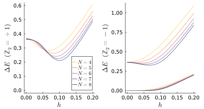
FIG. 4. Gaps to the first excited states above the ground state in the \mathbb{Z}_2 -even (left panel) and \mathbb{Z}_2 -odd (right panel) sectors. The even sector is gapped on either side of the transition. In the odd sector, we can observe the ground state degeneracy being lifted across the transition, while the next excited state also has a finite gap in the ferromagnetic regime. The decrease (and subsequent closing in the thermodynamic limit) of the shown gaps is consistent with a continuous phase transition around h \sim 0.1 .
