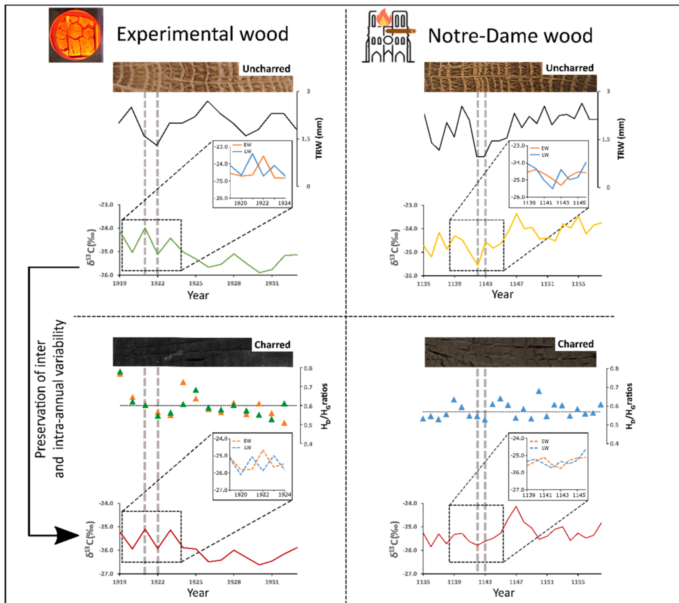
Fig 9. Schematic presentation of the different parameters incorporated in this study to investigate the preservation of the \delta^{13}\text{C} inter and intra-annual variability after carbonisation.
