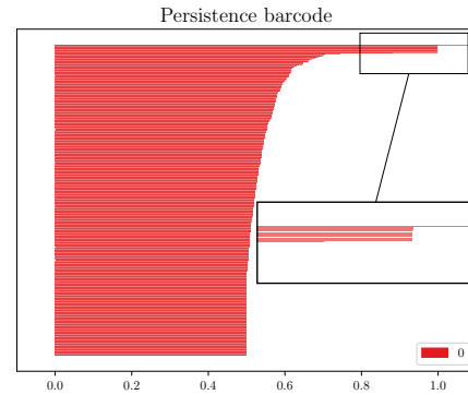
Fig. 4. Persistence Barcode. The zoomed-in region shows the stable region we are interested in. In a stable region, the number of connected components does not change in the specific interval, meaning that, most probably, those clusters carry some geometric meaning since \epsilon needs to change a lot before collapsing connected components.
