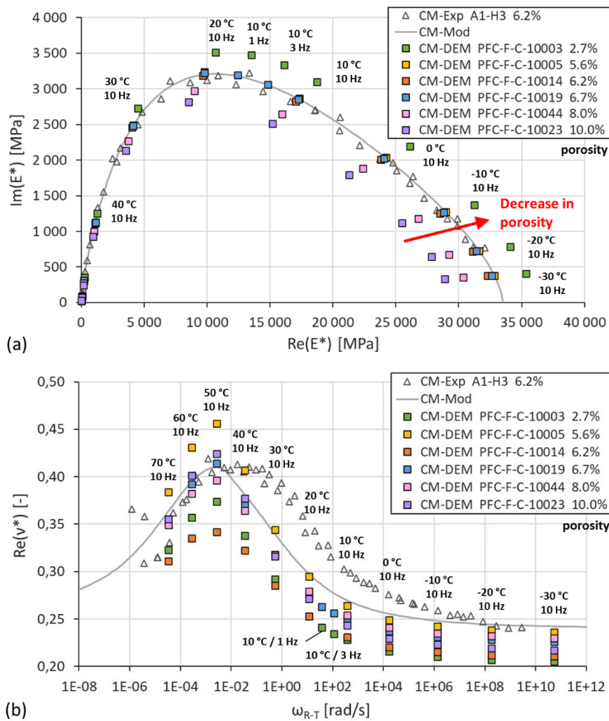
Fig. 3. FREIRE's asphalt concrete – Specimen A1-H3 (CM, 50 μm/m). Effect of numerical porosity in DEM on the complex stiffness modulus in the Cole-Cole plane (a) and on the real part Re(v^*) of the complex Poisson's ratio (b). Superposition of experimental data "Exp", analytical model VENoL "Mod" and DEM simulations.
