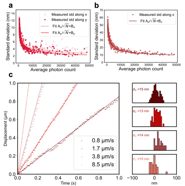
Figure 3. Localization precision of fixed Nano2Track-840/650 nanoparticles in the plane orthogonal to the optical axis (a) and along the optical axis (b). In both experiments, incident power is 4 mW. Experimental data are fitted with a B+A/\sqrt{N} law. Fit parameters: A_x = 218 et B_x = 1.8 nm, A_y = 236 et B_y = 1.2 nm, A_z = 1159 et B_z = 4.7 nm (c) Left: tracks of a nanoparticle moved by a piezo stage at different velocities. The dots stand for the measured displacements and the plain lines for the piezo-stage programmed motions. The incident power is 1 mW. (c) Right: histograms of the errors to the piezo-stage positions. The indicated localization precisions \sigma_x of the moving particle are estimated by standard deviations of the distributions of errors. The standard deviations are around 15 nm for all
