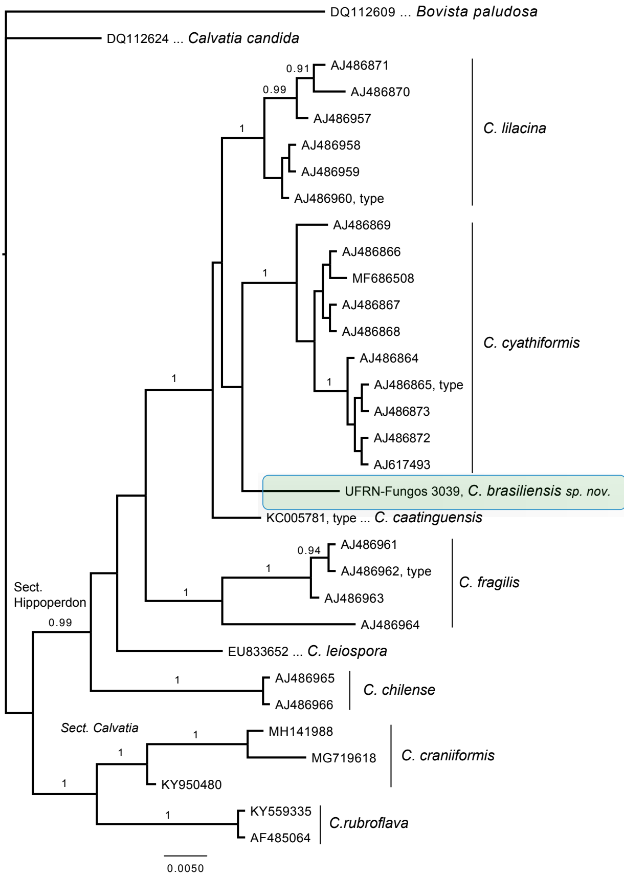
FP913 ITS nrDNA phylogenetic tree obtained with MrBayes v. 3.1.2 (Huelsenbeck & Ronquist 2001) under T92+G model for 5 M generations. The new species is marked with a rectangle. The posterior probabilities greater than 0.9 are indicated on the branches. Bovista paludosa was included as outgroup. Figtree v. 1.42 and Adobe Illustrator CS5 software were used to edit the final tree.
