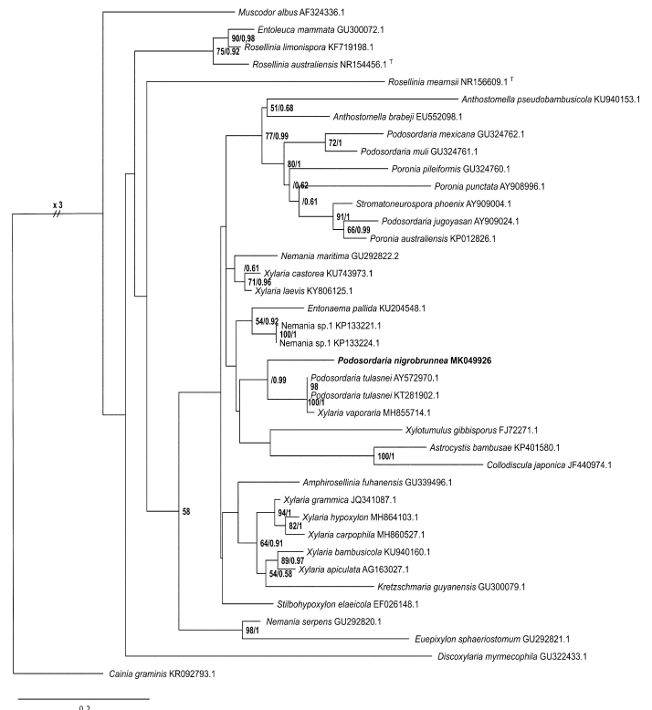
Maximum Likelihood tree inferred with RAXML-HPC BlackBox v. 8.2.10 from the ITS region. Bootstrap support (BS) values ≥ 50 % and Bayesian posterior probabilities (PP) ≥ 0.5 are displayed at the nodes as BS/PP. GenBank accession numbers are indicated behind the species names. Bar represents the expected substitutions per site. Type strains are indicated with superscript †. The novel species is indicated in bold. Alignment and tree in TreeBASE under 23082.
