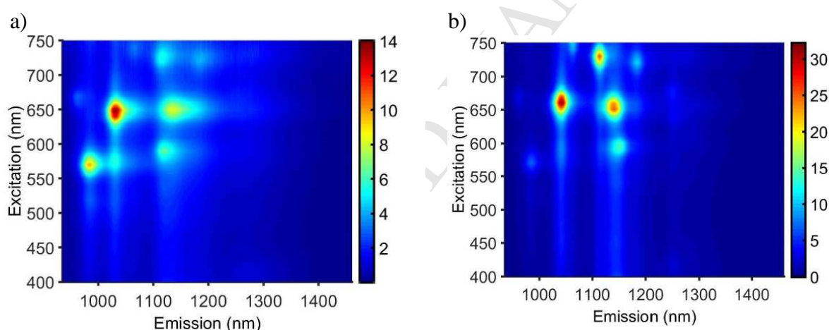
Figure 6: PL signal intensity versus emission (x-axis) and excitation (y-axis) of NT09 (a) and 4T@NT09 (b)
