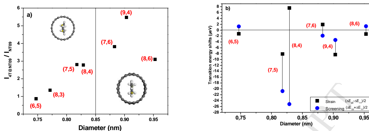
Figure 7: a) PL intensity ratio between 4T@NT09 and NT09 as a function of CNT diameters b) Mechanical and electronic contributions of the PL energy shifts for 4T@NT09 with respect to NT09
