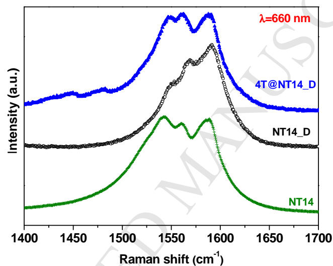
Figure 4: Raman spectra of annealed M_CNT14 (green cross), defective nanotube CNT14_D (open circle) and hybrid 4T@NT14_D (blue triangle)
