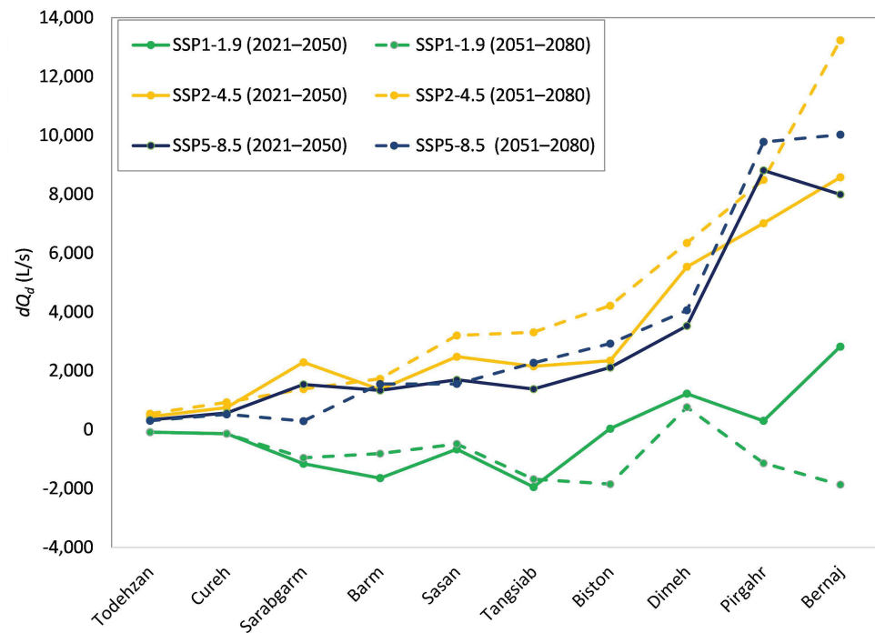
Figure 8. dQ_d value changes in terms of L/s in springs based on climate change scenarios SSP1-1.9, SSP2-4.5 and SSP5-8.5 in two time periods of the near future (2050–2021) and distant (2080–2051).
