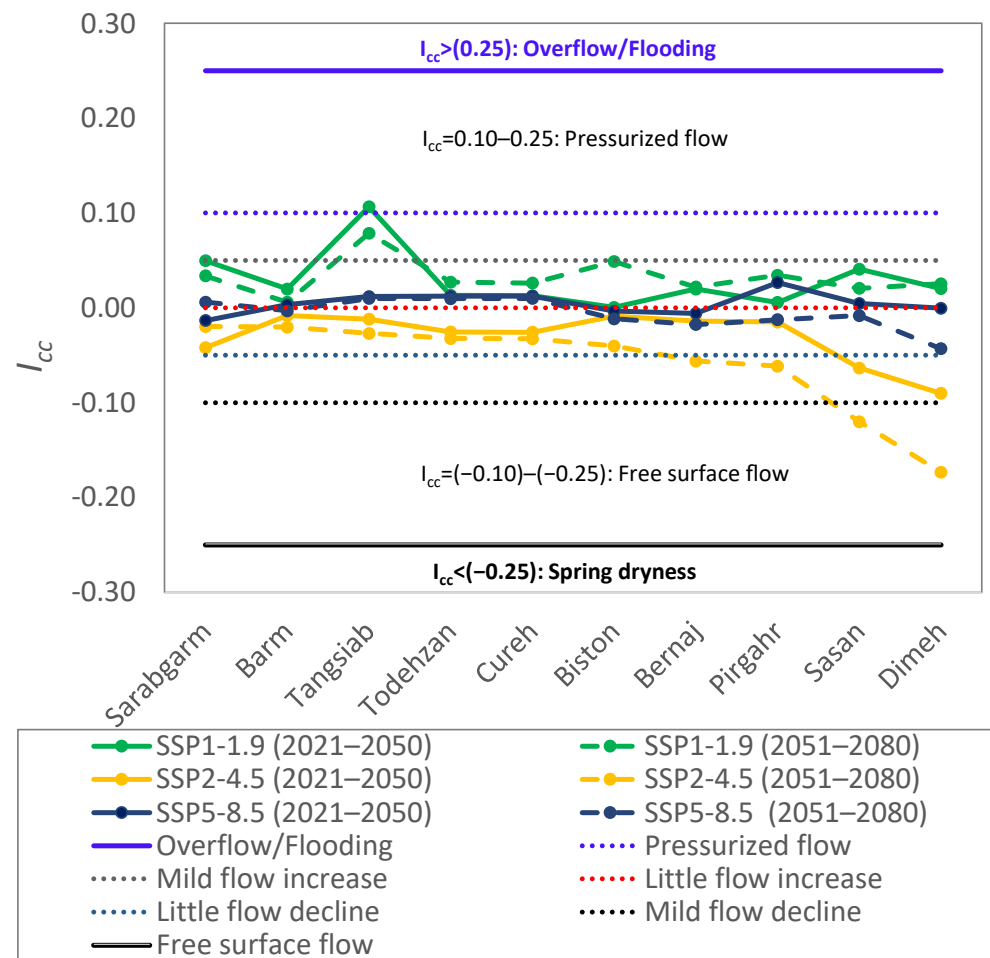
Figure 10. I_{cc} in springs under SSP1-1.9, SSP2-4.5, and SSP5-8.5 in two time periods of the near future (2050–2021) and far future (2080–2051). See Figure 3 for the concept of different terms of flow regime.
