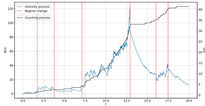
Figure 1: Representation of a Markov-Modulated Hawkes Process (MMHP) featuring an exponential Hawkes process intertwined with a two-state Markov chain.
