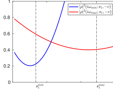
Fig. 7 Example of |\rho_h(i\omega_{\min}; s_1, -c)|^2 and |\rho_h(i\omega_{\max}; s_1, -c)|^2 as functions of s_1 .
