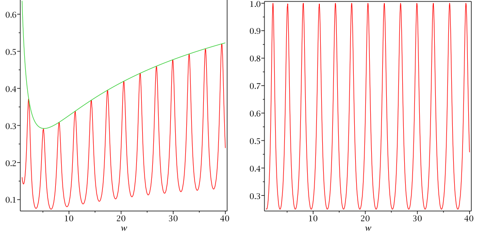
Fig. 5 Case s_2 = -c . Left: plot of |\rho|^2 and |\rho_h|^2 in the simplified situation where the diffusive domain is unbounded, as functions of \tau = i\omega . Right: corresponding plot for |\rho_w|^2 .
