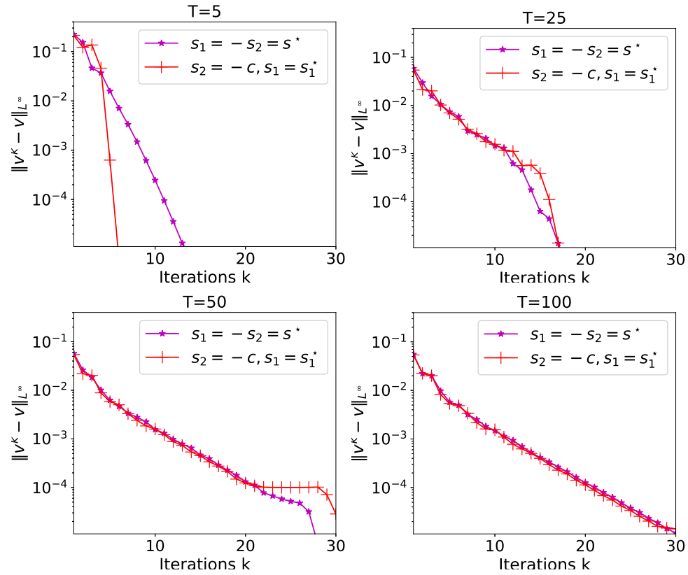
Fig. 13 Errors for longer time T = 5, 25, 50 and 100 with s_1 = -s_2 = s^* from the first optimization choice and s_2 = -c and s_1 = s_1^* from the second optimization choice.
