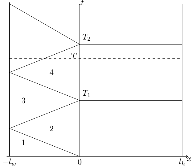
Fig. 4 Convergence in a finite number of steps due to the wave domain when s_2 = -c .
