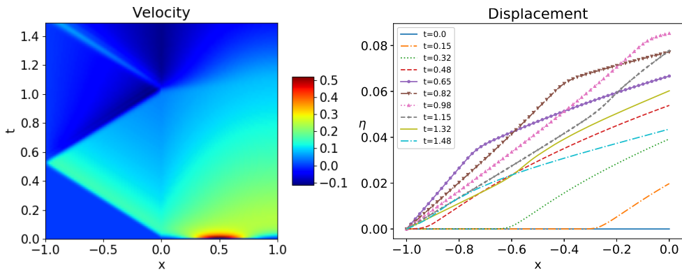
Fig. 9 As in Figure 8, but now with initial data supported in the heat domain.
