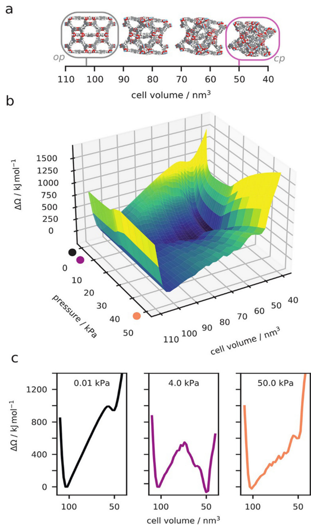
Fig. 6 Computed osmotic surface of methane adsorption on DUT-49 at 120 K, as a function of unit cell volume (a) and methane gas pressure (b). Examples of the 1D osmotic surface at specific gas pressures (c). Reproduced and adapted with permission from ref. 26. Copyright American Chemical Society 2021.
