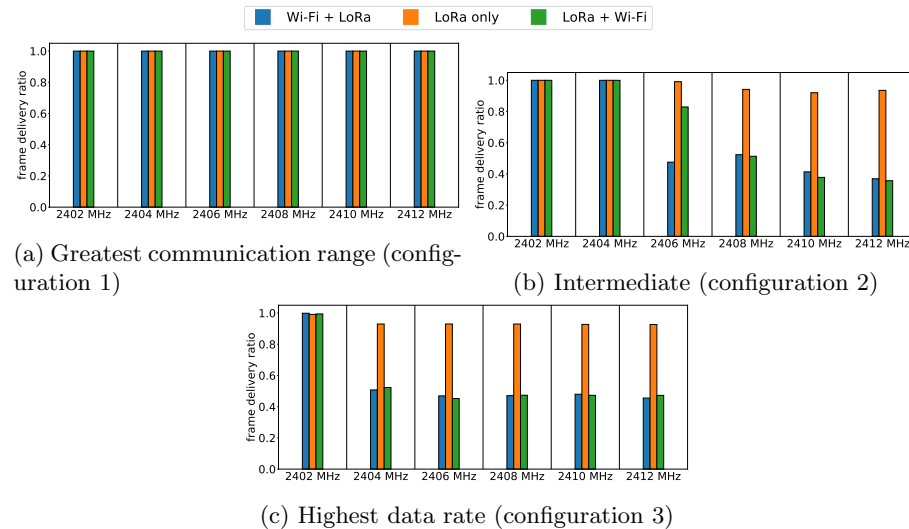
Figure 9: LoRa FDR depending on the center frequency.
