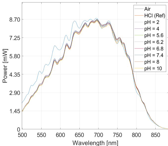
Fig. 6. Spectral response of bare TCF to pH variation.
