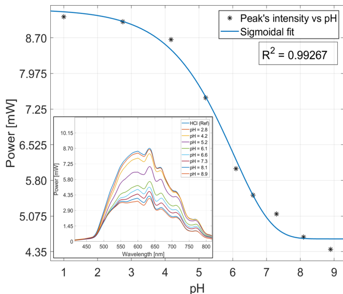
Fig. 7. Response of PAni-coated TCF sensor to pH variations. Inset: spectral evolution.
