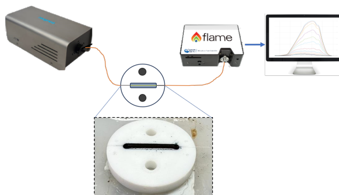
Fig. 3. Experimental setup of the novel fiber-optic pH sensor.
