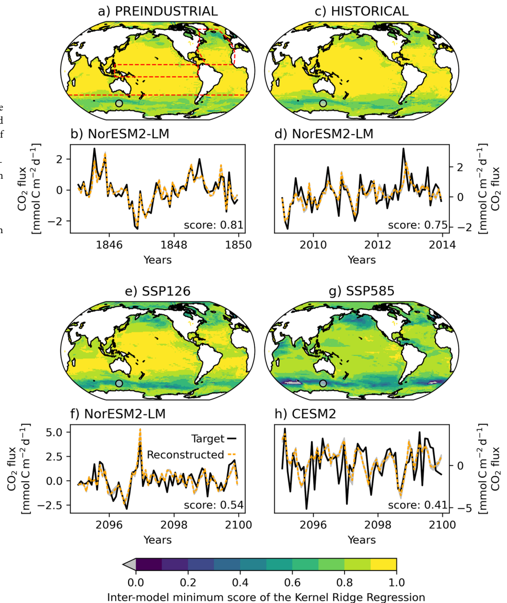
Fig. 2 | Ability of the kernel ridge regression in reproducing the original CO 2 flux inter-annual variability. Inter-model minimum score of the kernel ridge regression in (a) the preindustrial, (c) the historical, (e) the SSP126 and (g) the SSP585 scenarios. b, d, f, h show 5 years of the de-trended and de-seasonalized CO 2 flux time-series from the ESM with the lowest score (black lines) and from the kernel ridge regression reconstruction (dashed gold lines). Grey shading shows the standard deviation of the reconstructed CO 2 flux derived using bootstrapping. Shown are the 5 last years of the simulations from a single grid point in the Southern Ocean (grey point in the maps). In a), red dashed lines indicate regions with special focus in the analysis: the North Atlantic (10°N to 70°N), the equatorial Pacific (10°S to 10°N) and the Southern Ocean (south of 40°S).
