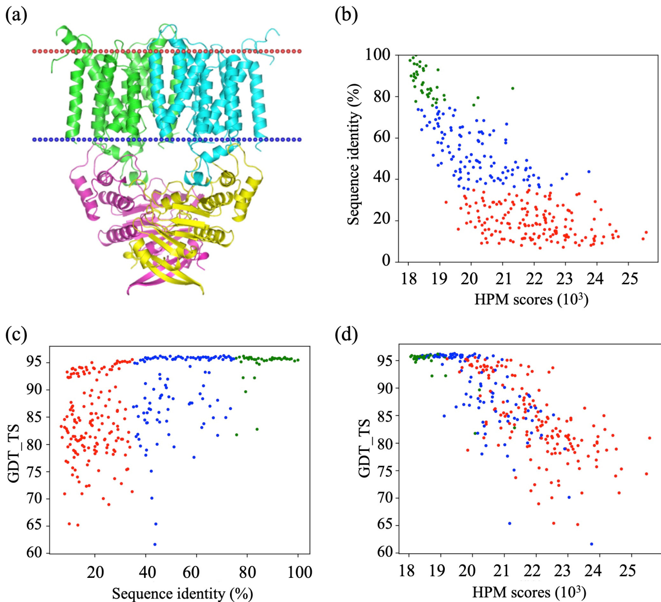
Figure 2. Example of putative metal-chelate type ABC transporter (PDB ID 2NQ2). (a) Three-dimensional visualization, (b) sequence identity of the alignments (%) vs. HPM scores (10 3 ), (c) GDT_TS vs. sequence identity of the alignments (%), and (d) GDT vs. HPM scores (10 3 ). (b–d) good alignment (green), intermediate alignment (blue) and bad alignment (red).
