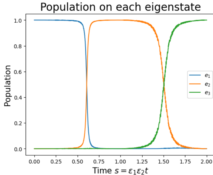
Figure 3: Simulations for \alpha = 0.5 , \beta = 6 , \epsilon_1 = 10^{-4/3} , \epsilon_2 = 10^{-3} : Population inversions between (\mathbf{e}_1, \mathbf{e}_2) and (\mathbf{e}_2, \mathbf{e}_3) happen successively.
