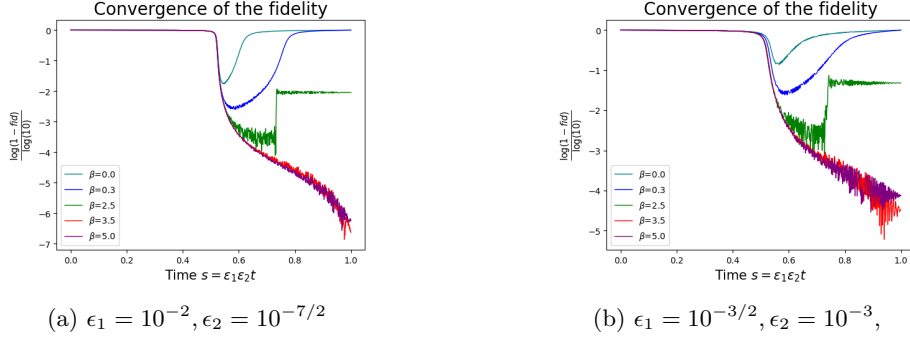
Figure 2: Simulations for \alpha = 0.3 , \beta \in \{0.0, 0.3, 2.5, 3.5, 5.0\} : Convergence holds when both first-order and second-order conditions are satisfied and is lost when the first-order condition is violated. Notice that for \beta = 2.5 an abrupt variation of the fidelity (in the log scale) occurs when \lambda_3(\alpha, \beta) - \lambda_2(\alpha, \beta) - 2f(s) = 0 , that is, at s = \arccos(-2/3)/\pi \approx 0.7323 .
