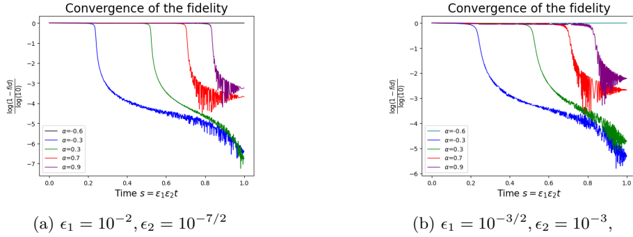
Figure 1: Simulations for \beta = 6 , \alpha \in \{-0.6, -0.3, 0.3, 0.7, 0.9\} : Convergence holds only when the first-order condition (Hypothesis 1) is satisfied and the best convergence is obtained when both the first-order condition and the second-order condition (Hypothesis 1 and Hypothesis 2) are satisfied.
