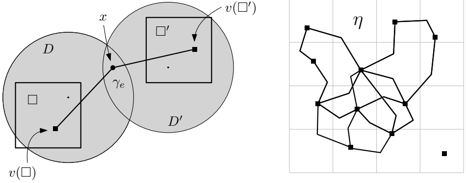
Fig. 2. Illustrating the drawing \eta . The left part is the construction of one edge curve \gamma_e and the right part is an example of how the drawing \eta finally looks like.
