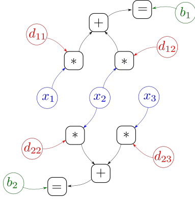
Fig. 8. The constraint network has no cycle (it is a tree). Thus the interval propagation is minimal
