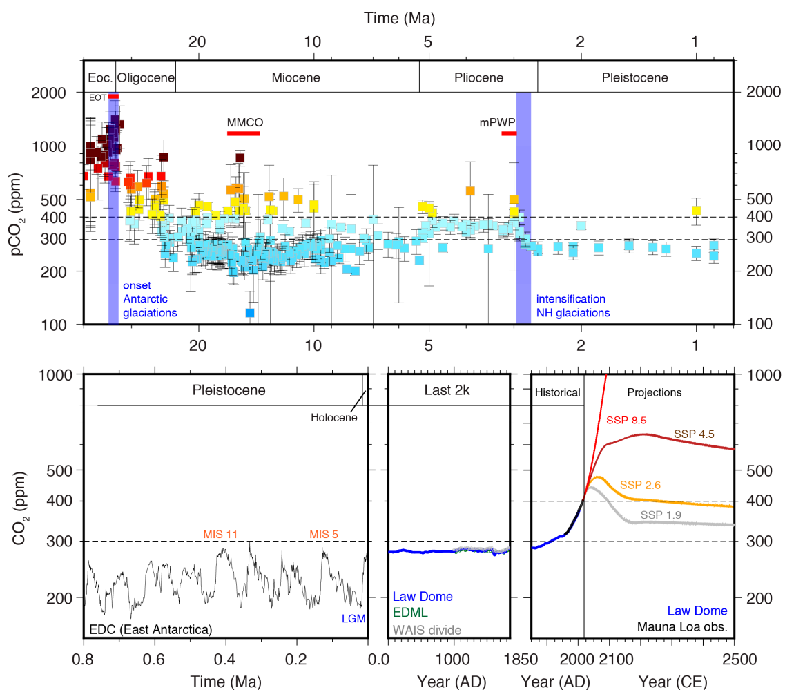
Figure 1. Evolution of atmospheric CO 2 concentration from deep past to future. Deep past pCO 2 level reconstructions are from sediment cores [39]; Pleistocene CO 2 reconstruction is from EPICA Dome C (East Antarctica [36]); the last 2k CO 2 reconstructions are from Law dome (East Antarctica, [55]), Drauning Maud Land [56] and West Antarctic Divide (WAIS, [57]); Historical CO 2 concentration is from law Dome (West Antarctica); 20 th century CO 2 concentration are from the Mauna Loa observatory; Projected CO 2 pathways correspond to the new Shared Socio-Economical pathways (SSP, [58]) as used in CMIP6. The main warm periods of interest are indicated on the frames (see Table 1). Blue bars indicate the onset of Antarctic glaciations at the EOT boundary and the intensification of Northern Hemisphere (NH) glaciations at the Plio-Pleistocene transition, respectively.
