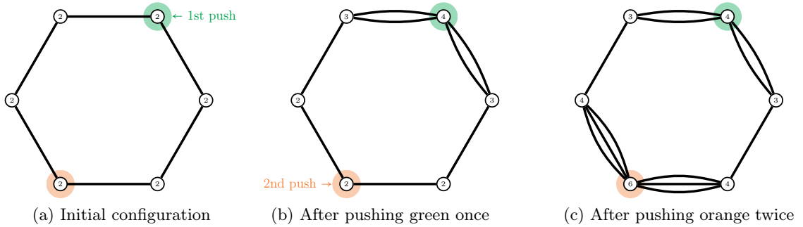
Figure 1: Sequential construction of a proper pushing scheme of C_6 . From the initial configuration (a), the vertex highlighted with green is pushed once, resulting in (b). Then, the vertex highlighted with orange is pushed twice, resulting in (c). It can be checked (numbers in vertices indicate their degrees) that the resulting multigraph is locally irregular, and thus that the depicted pushing scheme is indeed proper. Due to this proper pushing scheme, we have P^t(C_6) \leq 3 and P^1(C_6) \leq 2 .
