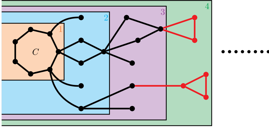
Figure 2: An example of ordering in which the vertices of a cactus are pushed, in the proof of Theorem 3.7. Vertices of an initial cycle C are pushed first, before the vertices of distant configurations get also pushed, accordingly to their distance to C and to the 2-degenerate structure of the cactus. Structures in red are problematic end-structures, for which we may not fulfil the desired sums modulo 3.
