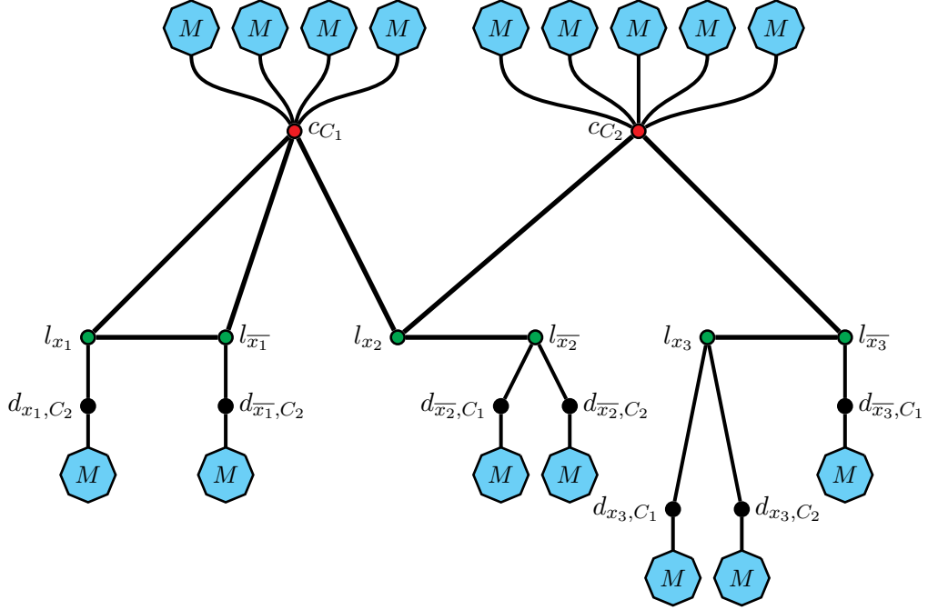
Figure 4: Illustration of the reduction in the proof of Theorem 4.2, for the formula F = C_1 \wedge C_2 where C_1 = (x_1 \vee \bar{x}_1 \vee x_2) and C_2 = (x_2 \vee x_2 \vee \bar{x}_3) (the set of variables being thus \{x_1, x_2, x_3\} ). Red vertices are clause vertices, while green vertices are literal vertices. Blue octagonal shapes with an “M” inside indicate where M -gadgets are attached.
