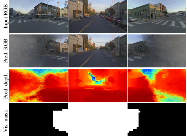
Figure 4. Visualization of the visibility grid (Sec. 3.5). Predictions done with the NeRF trained by front camera on a Pandaset [44] sequence.
