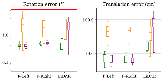
Figure 7. Results on Pandaset [44] for SOAC, MOISST [12] and SOAC w/o semantic filtering as box plots with log scale, the red lines show the initial error (best viewed in color).
