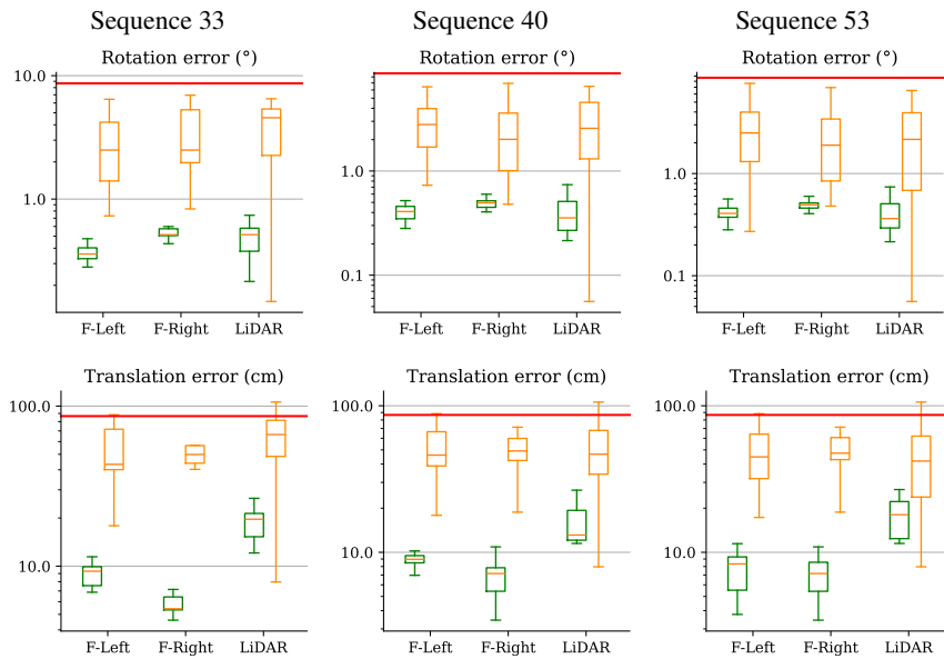
Figure 13. Results for Pandaset [29] per sequence for SOAC and MOISST [12] as box plots with log scale. The red lines show the initial error (best viewed in color).
