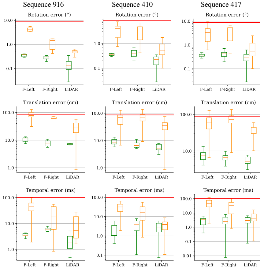
Figure 14. Results for nuScenes [3] per sequence for SOAC and MOISST [12] as box plots with log scale. The red lines show the initial error (best viewed in color).
