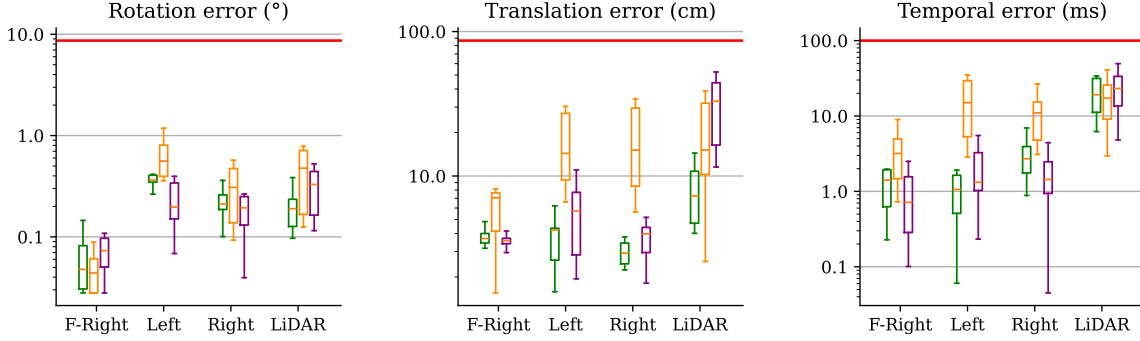
Figure 11. Ablation results on KITTI-360 [18] sequence 4: for SOAC, SOAC w/o Sigmoid and SOAC w/o visibility grid as box plots with log scale, the red lines show the initial error (Best viewed in color).
