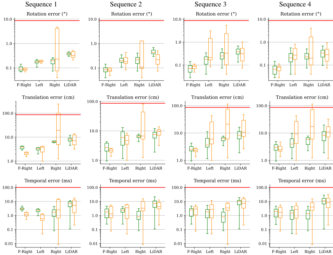
Figure 12. Results for KITTI-360 [18] per sequence for SOAC and MOISST [12] as box plots with log scale. The red lines show the initial error (best viewed in color).
