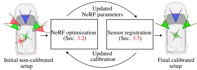
Figure 1. Method overview. SOAC is a novel multimodal spatio-temporal calibration method for cameras and LiDAR in the context of autonomous driving. By alternating the training of multiple implicit scenes (Sec. 3.2) and sensors co-registration from these representations (Sec. 3.3), SOAC achieves precise self-supervised calibration from raw data acquired in unconstrained urban environments.
