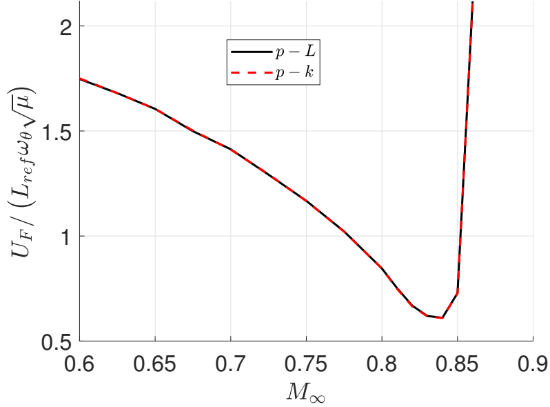
Figure 2: Flutter speed index U_F / (\omega_\theta L_{ref} \omega_\theta \sqrt{\mu}) against the Mach number M_\infty for the Isogai case A [29] as obtained by the p-k and p-L methods.
