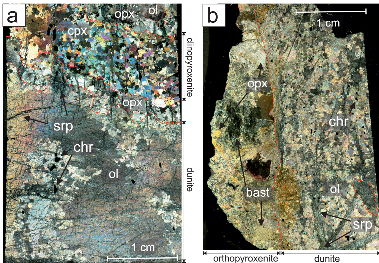
Fig. 3 Petrographic features of host dunite and pyroxenitic veins. a - Microphotograph of a thin section of dunite KH53 with clinopyroxenite vein (crossed-polars). Note the presence of orthopyroxene screen at the contact with the host dunite. b - Microphotomicrograph of dunite KP10A with orthopyroxenite vein; dunite comprise porphyroclasts of olivine (one marked with dashed lines), serpentine locally form channel-like structures (crossed-polars). Mineral abbreviations: ol – olivine, chr – chromite, opx – orthopyroxene, cpx – clinopyroxene, srp – serpentines, bast – bastite.
