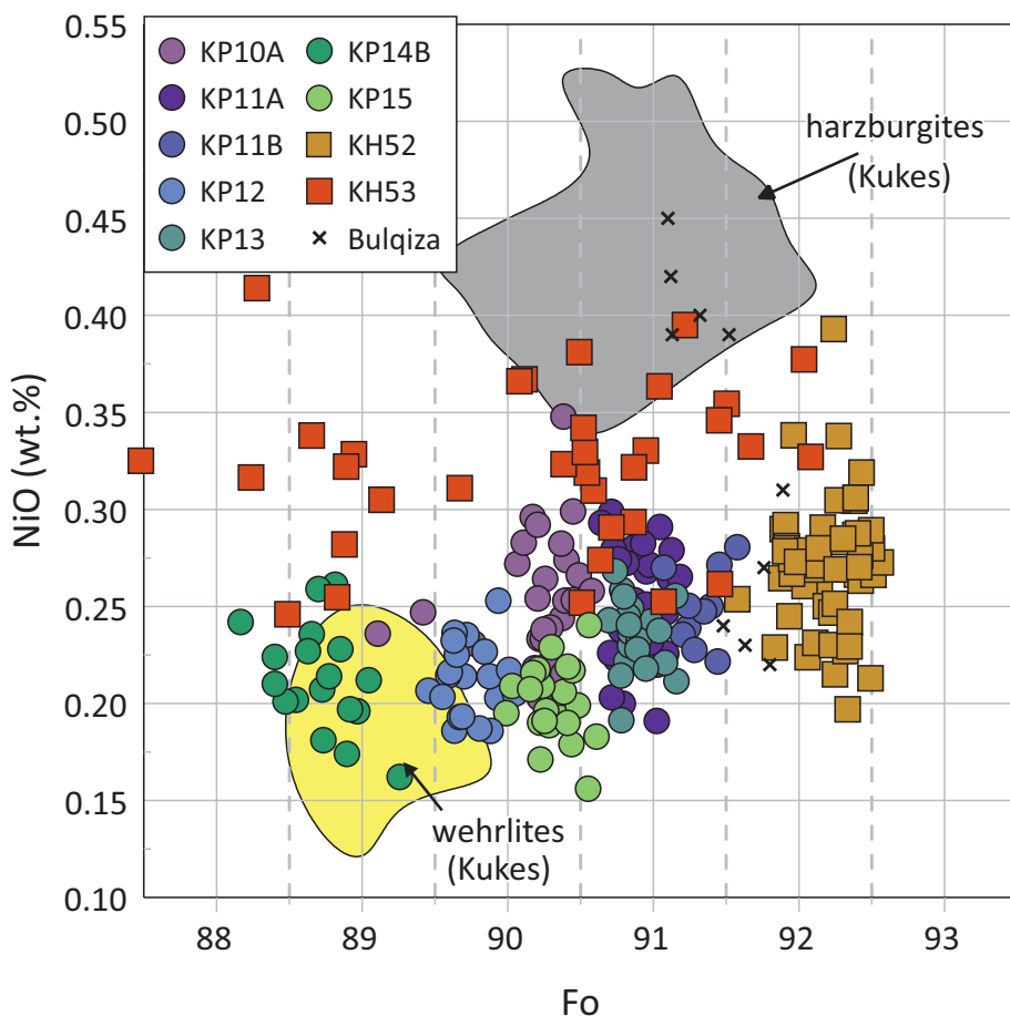
Fig. 6 Forsterite – NiO relations in olivine. “harzburgites” and “wehrlites” fields mark composition range of olivine from those rocks within Kukes massif (J. Mikrut unpublished data). Circles mark samples collected from the profile, squares – additional two samples with complete veins cross-sections.
