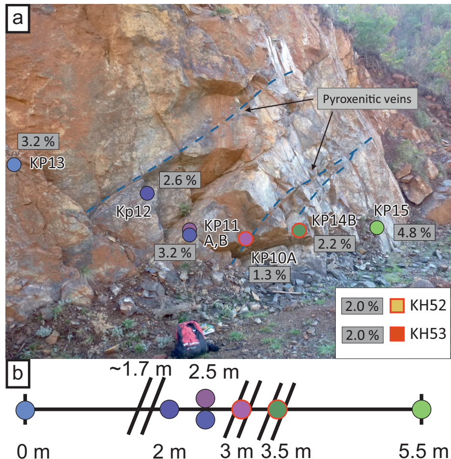
Fig. 2 Field relationships between veins and the host dunite. a - Occurrence of the veins in the studied outcrop with sample locations. Symbols with bold red edge represent dunites with pyroxenitic veins. Numbers in grey fields indicate modal content of spinel. b - Schematic profile showing spatial relationships between samples. Parallel lines marks pyroxenitic veins.
