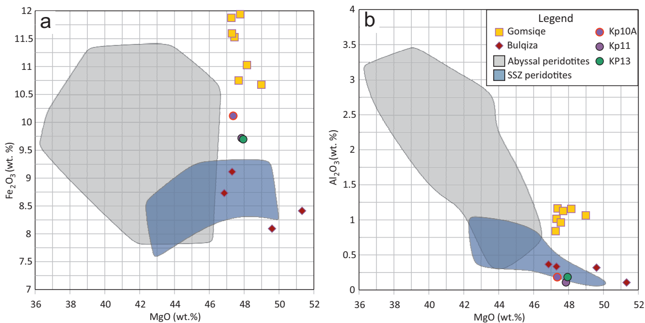
Fig. 9 Bulk rock chemical composition of Kukes dunites. a – Relations between MgO and Fe 2 O 3 contents. b – Relations between MgO and Al 2 O 3 contents. Abyssal peridotites field after Niu (2004), data for SSZ peridotites is from Parkinson and Pearce (1998), data for Gomsiqe dunites (western Mirdita) from Wu et al. (2022) and for Bulqiza dunites (eastern Mirdita) from Xiong et al. (2015). All literature data was recalculated to Fe 2 O 3 and volatile-free composition.
