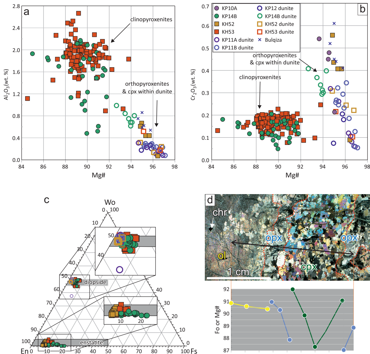
Fig. 7 Chemical features of clinopyroxene (a, b), classification of pyroxenes (c) and chemical profile across clinopyroxenitic vein (d). a - Relations between Mg# and Al_2O_3 content. b - Relations between Mg# and Cr_2O_3 content c - Pyroxene ternary classification diagram, showing composition of both clino- and orthopyroxene. d - Chemical profile across clinopyroxenitic vein, orthopyroxene screen and contacting dunite (KH53) showing variation of Fo in olivine and Mg# in pyroxenes contents. Solid symbols indicate analyses performed within the veins, open symbols represent analyses of interstitial clinopyroxene within dunite. Data for clinopyroxene from Bulqiza dunite is from Xiong et al. (2015).
