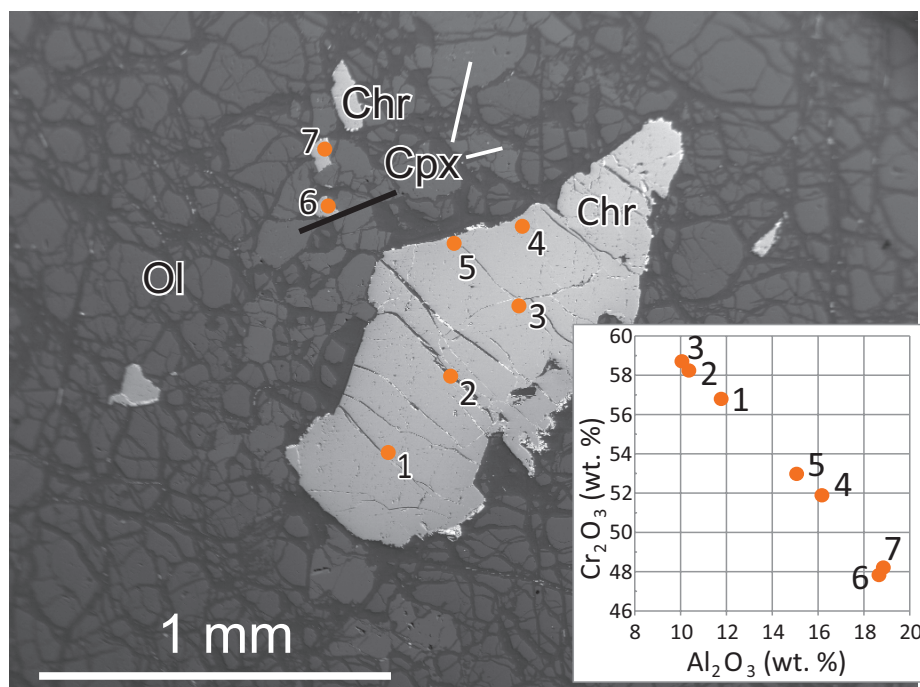
Fig. 4 Backscattered electron image of a large chromite grain from sample KP14B. Note the presence of small interstitial clinopyroxene. Inset diagram shows variability of Cr 2 O 3 and Al 2 O 3 content within chromite grains, analytical spots locations correspond to the points on the diagram.
