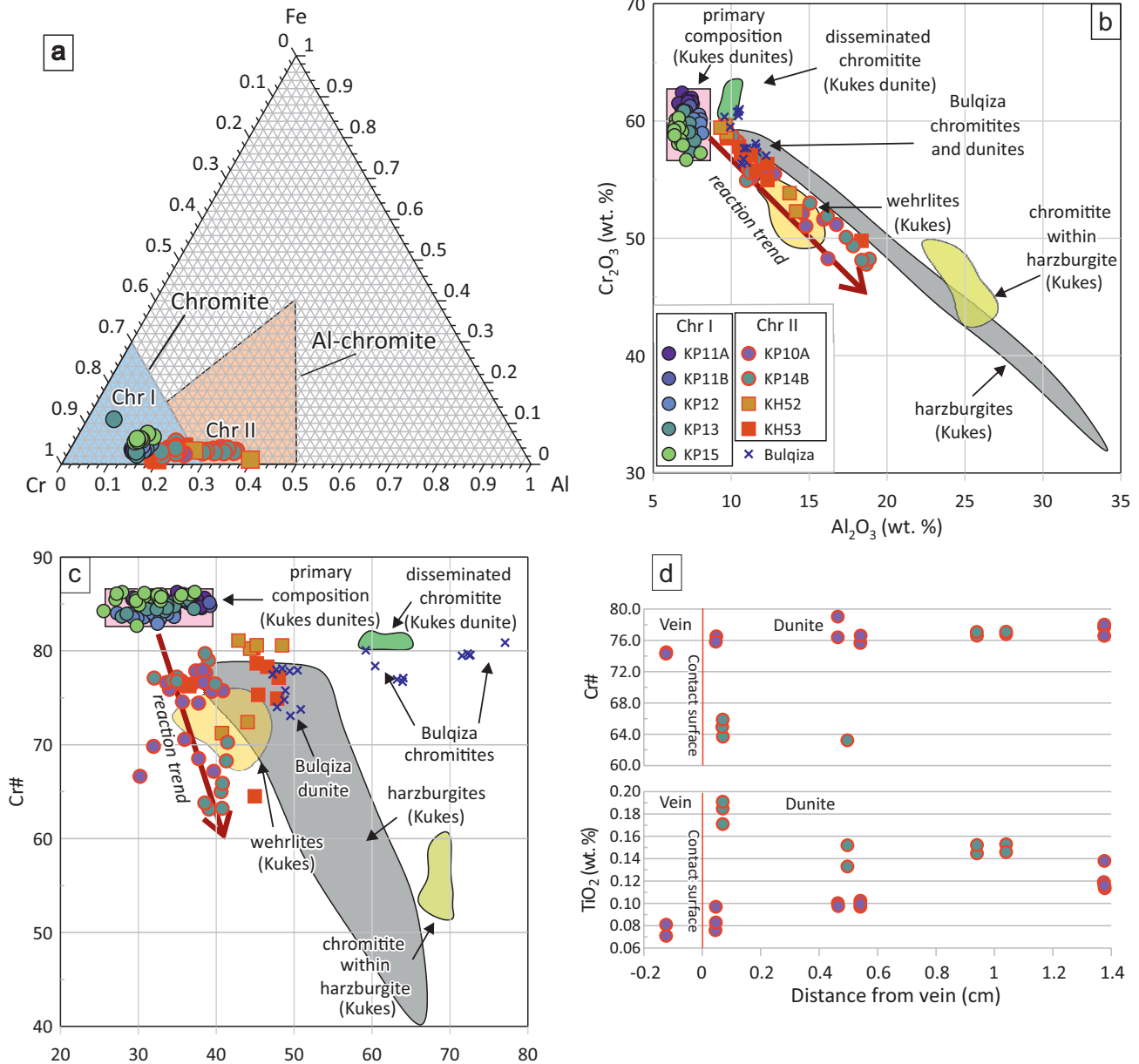
Fig. 5 Chemical composition of spinel. a – Ternary classification diagram of spinels. b – Relation between Al_2O_3 and Cr_2O_3 contents. c – Cr# – Mg# relationships. d – Profiles illustrating Cr# and TiO_2 contents in samples KP10A and KP14B changing with the distance from pyroxenitic veins; “harzburgites”, “wehrlites” and “chromitites” fields mark composition range of spinel from those rocks within the whole Kukes massif (J. Mikrut unpublished data), data for Bulqiza is from Xiong et al. 2015.
