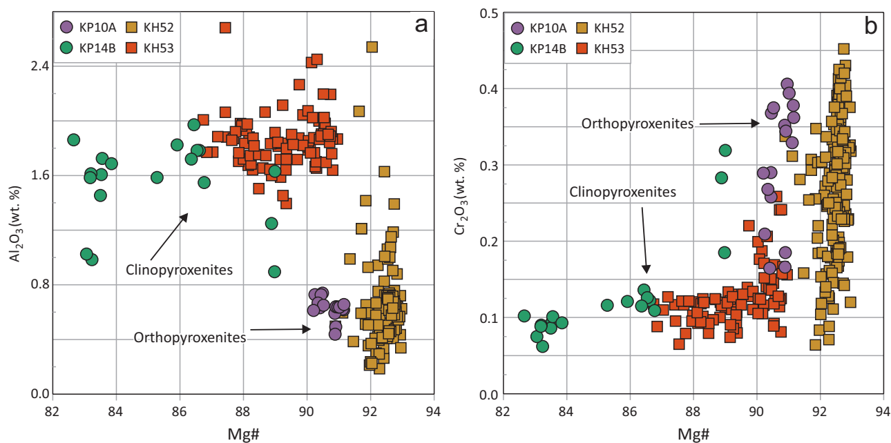
Fig. 8 Chemical composition of orthopyroxene. a - Relations between Mg# and Al 2 O 3 content. b - Relations between Mg# and Cr 2 O 3 content. All analyses performed on vein pyroxene.
