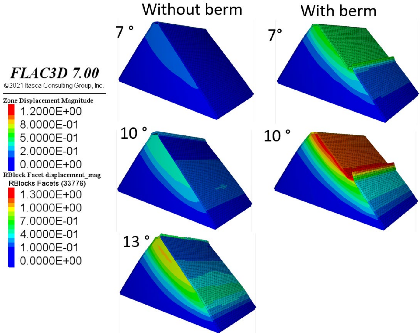
Fig. 7: Displacements of the studied rockfill dams with dry-stone pitching at several rotation angles before failure: without berm (left) and with berm (right)
