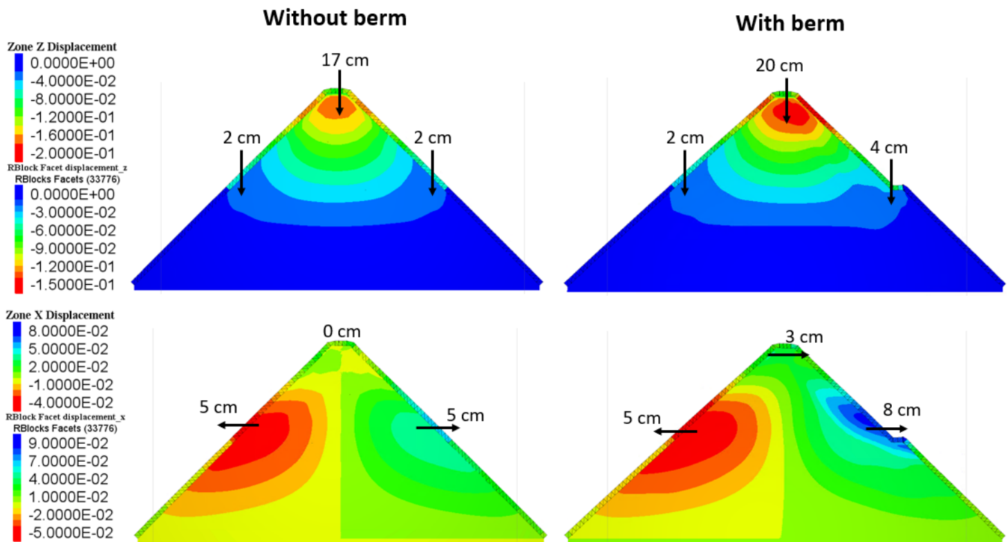
Fig. 6: Vertical and horizontal displacements at the end of construction of a rockfill dam with dry-stone pitching: without berm (left) and with berm (right)
