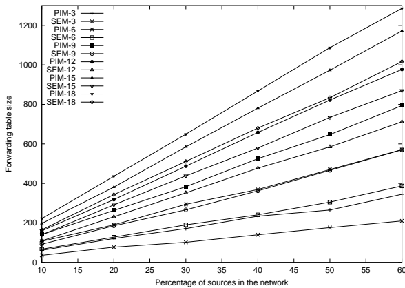
Fig. 4. Forwarding table size - Waxman model
