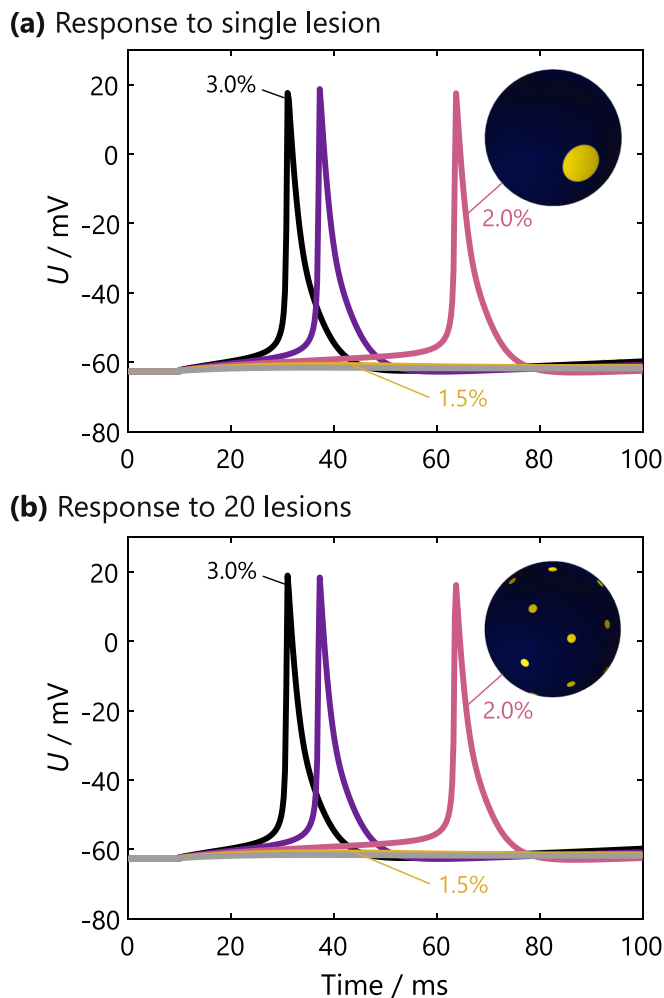
Fig. 10. Response to lipid oxidation in the whole-cell model. As example, lesion(s) consisting of 20 % PoxnoPC are considered to form at time t = 10 ms. (a) Response to creation of a single lesion with area of 1.0, 1.5, 2.0, 2.5, or 3.0 % of the cell membrane area. AP triggers for area \geq 2.0 % of the cell membrane area. (b) Response to creation of 20 lesions with their total (summed) area of 1.0, 1.5, 2.0, 2.5, or 3.0 % of the cell membrane area. The inset in each graph depicts a cell with either (a) single or (b) 20 oxidized lesions (yellow) with the total lesion area accounting for 2.0 % of the cell membrane.
