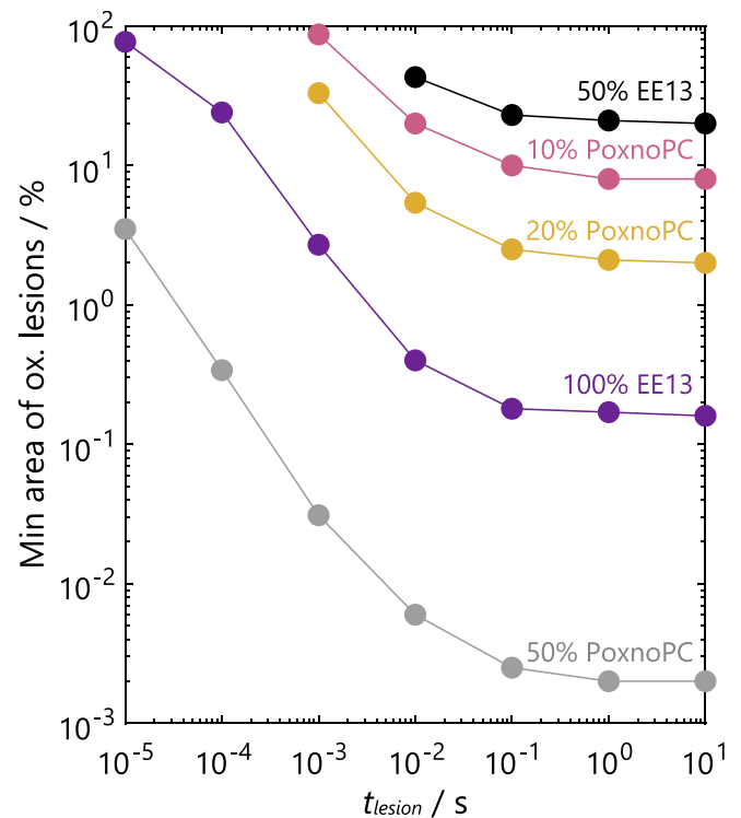
Fig. 11. Minimum areal fraction of oxidized lesions required to trigger an AP, depending on the characteristic decay time t_{lesion} , with which the membrane properties return to baseline value.
