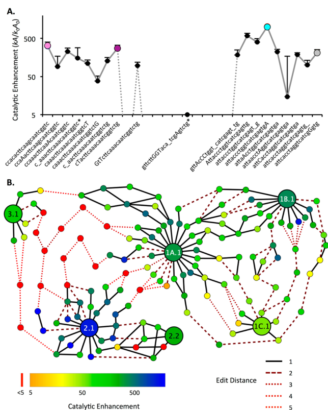
Figure 4. Evolutionary pathways for aminoacylation ribozymes. (A) Catalytic enhancement along a best pathway discovered from the center of Family 1B.1 (pink, S-1B.1-a), to 1A.1 (purple, S-1A.1-a), to 2.1 (cyan, S-2.1-a), to 2.2 (gray, S-2.2-a). Capital letters denote sequence positions changing at each step; underscore indicates a deletion. A large drop in activity is required for several mutations between Motif 1 and Motif 2. Error bars are standard deviation from triplicate measurements (only top bar is shown). Also see Supporting Figure S11. Asterisk (*) indicates a sequence that was found in only one replicate (RS1). (B) Evolutionary network displaying the 10 best pathways discovered between the centers of six key families (1A.1, 1B.1, 1C.1, 2.1, 2.2, and 3.1) representing each motif and submotif and the two most active centers from Motif 2. Each node is an individual sequence with activity measured by k -Seq indicated by color (see legend; red indicates activity at or below the baseline rate). The lines indicate mutational distance between sequences (solid black line = 1 mutation). Dotted lines indicate sequences at baseline activity (see legend). The majority (67%) of the edits along these pathways are substitutions; the remainder are indels.
