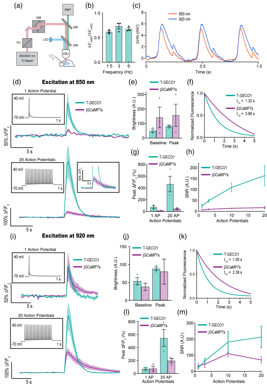
Fig. 4 Two-photon Ca 2+ imaging of T-GECO1 in organotypic hippocampal slices. (a) Schematic of the setup. PC = pockels cell, GM = galvo mirrors, and DM = dichroic mirror. (b) \Delta V_{m850} / \Delta V_{m920} ratio of ChromE-expressing organotypic hippocampal slices. (c) \Delta V_m for ChromE-expressing organotypic hippocampal slices induced by 850 or 920 nm laser illumination at 3 Hz. (d) Representative traces of T-GECO1 (teal) and jGCaMP7s (purple) for 1 action potential (top) and 20 action potentials (bottom) excited at 850 nm. (e) Baseline brightness (A.U.) for the two indicators at baseline (before stimulation) and at peak (maximum brightness after stimulation) at 850 nm excitation. (f) Normalized fluorescence decay for the two indicators at 850 nm excitation. (g) Peak \Delta F/F_0 (%) for the two indicators at 1 or 20 action potentials at 850 nm excitation. (h) SNR for the two indicators with respect to action potentials at 850 nm excitation. (i) Representative traces of T-GECO1 (teal) and jGCaMP7s (purple) for 1 action potential (top) and 20 action
