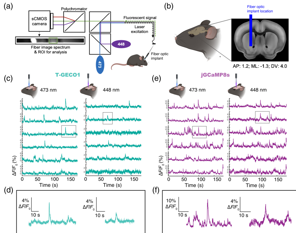
Fig. 5 In vivo Ca 2+ detection in the nucleus accumbens using fiber photometry. (a) Simplified schematic illustrating the fiber photometry setup, featuring two excitation wavelengths of 473 and 448 nm. (b) Precise position of the fiber optic implant. (c) Representative fluorescence traces of T-GECO1 at 473 nm excitation (left) and 448 nm excitation (right). (d) Zoomed-in view of the outlined traces displayed in (c). (e) Representative fluorescence traces of jRCaMP1e at 473 nm excitation (left) and 448 nm excitation (right). (f) Zoomed-in view of the outlined traces displayed in (e).
