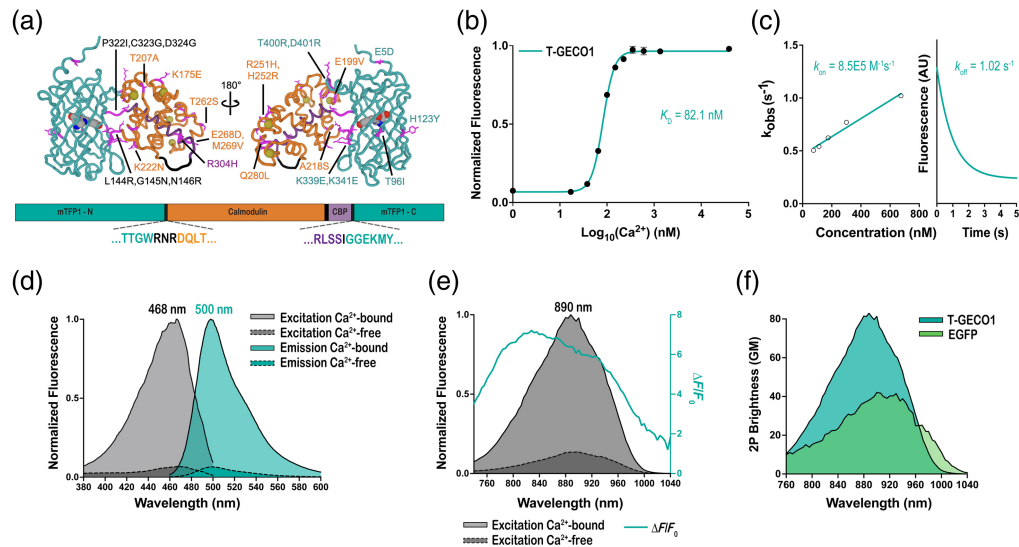
Fig. 1 Development and characterization of T-GECO1 as a purified protein. (a) Two views of the modeled structure of the Ca 2+ -bound state of T-GECO1. For the structure representation, mutated residues are shown as magenta sticks, Ca 2+ is shown as yellow spheres, and the chromophore is shown in space-filling representation. Both the protein structure and the labels are shown in teal for the mTFP1-derived domain, in orange for the CaM domain, in purple for the CaM-binding peptide, and in black for linkers. Colors are consistent with the sequence alignment shown in Fig. 2. The overall structure was predicted using ColabFold. 32 The chromophore was positioned using PyMol (Version 2.5.4 Schrödinger, LLC.) to superimpose the structure of mTFP1 (PDB ID 2HQK) 23 with the fluorescent protein portion of the T-GECO1 model. Ca 2+ ions were similarly positioned by superimposing the CaM domain of GCaMP2 (PDB ID 3EVR) 33 with the CaM portion of the T-GECO1 model. (b) Ca 2+ titration of T-GECO1. (c) Stopped-flow kinetic measurements of the fluorescence response of T-GECO1 for Ca 2+ association (left) and dissociation (right). (d) Excitation and emission spectra of T-GECO1 in the presence and absence of Ca 2+ . (e) Two-photon excitation-induced fluorescence of T-GECO1 as a function of wavelength, in the presence and absence of Ca 2+ , with \Delta F/F_0 represented in teal. (f) Two-photon cross-section of T-GECO1 in the Ca 2+ -bound state compared with the two-photon cross-section of EGFP.
