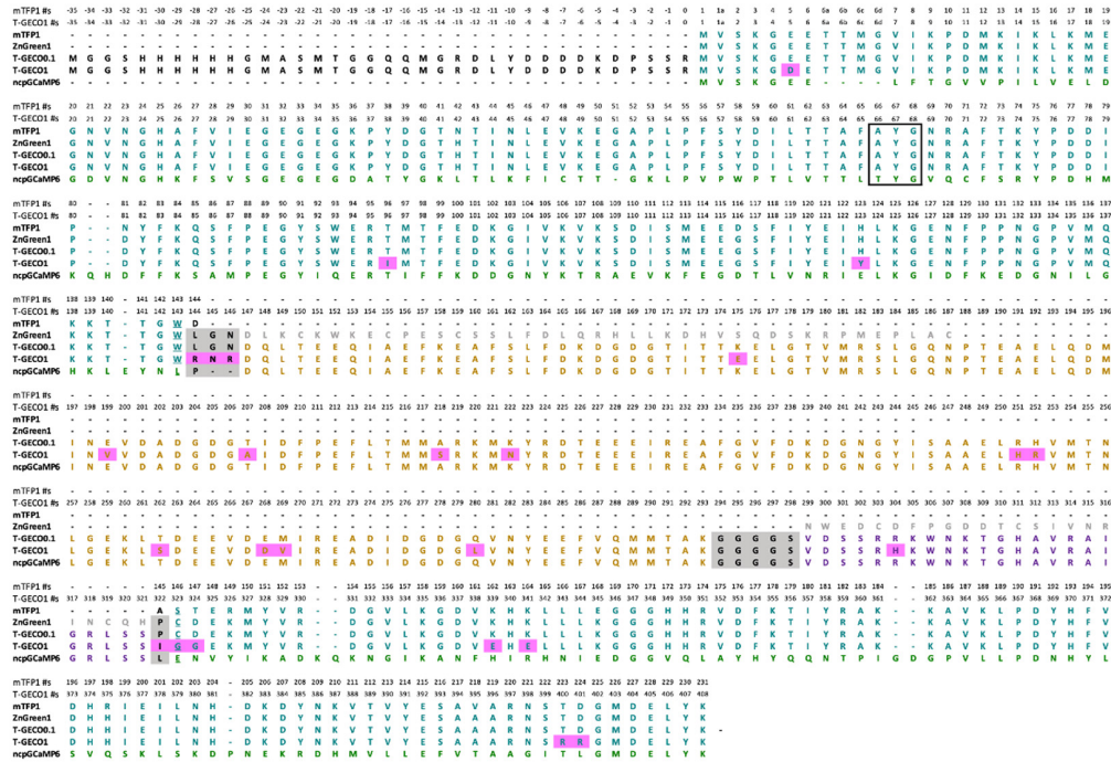
Fig. 2 Sequence alignment of T-GECO1 and related proteins. Residues are colored teal for the mTFP1-derived domain, orange for the CaM domain, purple for the CaM-binding peptide, and black on a gray background for the linkers. Mutated residues are shown on a magenta background. A black box encloses the chromophore-forming tripeptide. The gatepost residues 143 and 146 (using mTFP1 numbering) are underlined. 34 Colors are consistent with the structural model shown in Fig. 1(a).
