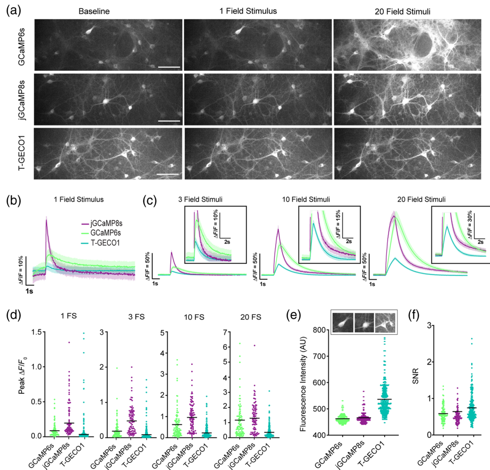
Fig. 3 Characterization of T-GECO1 in rat cultured neurons. (a) Images of primary rat hippocampal cultured neurons expressing GCaMP6s, jGCaMP8s, and T-GECO1 under the hSyn promoter at baseline and after field stimulations of 1 and 20 field stimulation (FS) pulses at room temperature. Scale bar, 100 \mu\text{m} . (b) Normalized \Delta F/F_0 traces for stimulations at 1 field stimulus and (c) 3 FS, 10 FS, and 20 FS at 30 Hz. (d) Peak \Delta F/F_0 of the three sensors across the same conditions. (e) Baseline brightness of the three sensors. (f) SNR for the three variants across conditions. Traces and error bars denote mean \pm s.e.m. Each data point is one ROI and is pooled across three independent wells.
