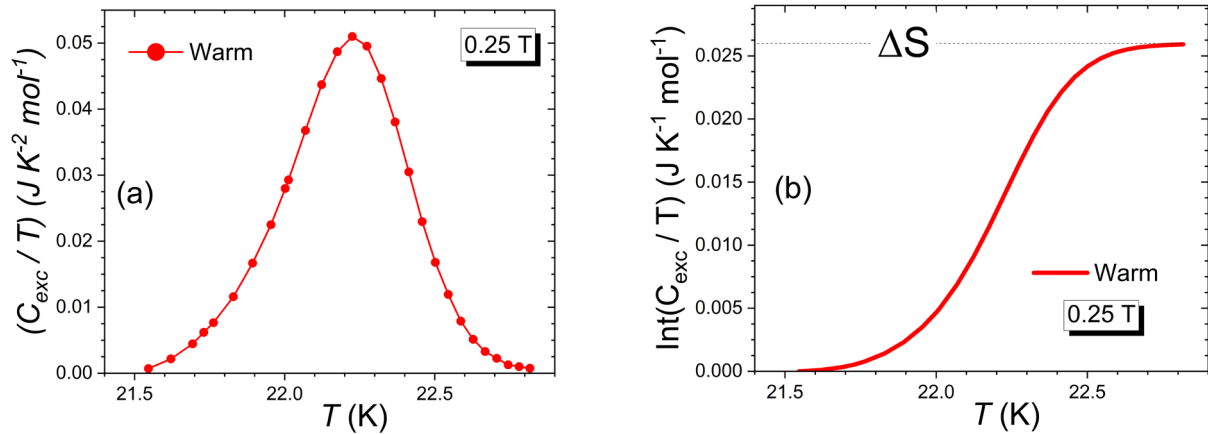
Fig. S13: (a) Ratio of the excess heat capacity to temperature around the transition in 0.25 T; (b) Integration of C_{\text{exc}}/T(T) across the transition; the saturation value reflects the entropy jump \Delta S .
