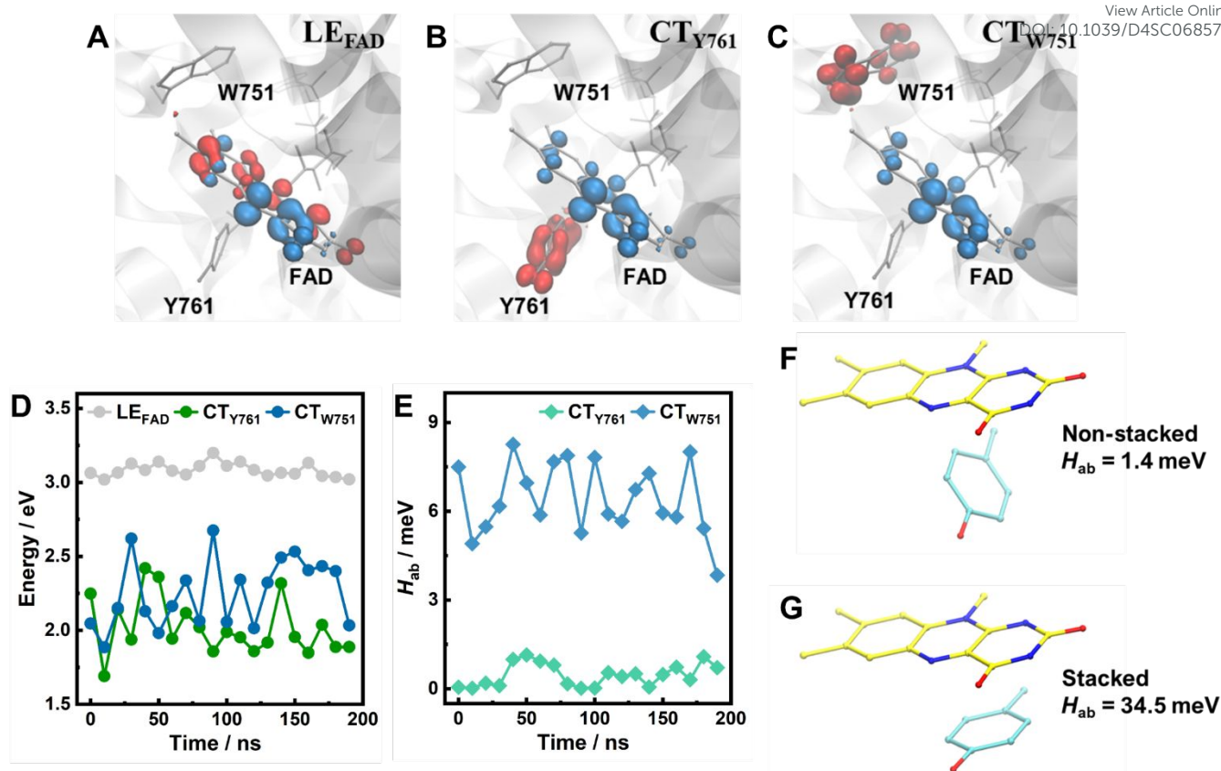
Fig. 4 (A, B and C) Hole–electron distributions of the FAD LE state (A), the lowest-lying CT states involving Y761 (B) and W751 (C). Red and blue regions denote the hole and electron distributions, respectively (isovalue = 0.004). Hydrogen atoms are not shown for clarity. (D, and E) The energy levels of these states (D), with respect to the electronic ground state, as well as the electronic couplings between the LE and CT states in WT LSD1 (E), along the MD trajectories. (F and G) Calculated electronic coupling between flavin LE state and tyrosine–flavin CT state in non-stacked (F) and stacked (G) donor–acceptor configurations but with similar separation distance (ca. 4 Å). Hydrogen atoms are not shown for clarity.
