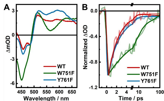
Fig. 3 Transient absorption spectra of LSD1 variants measured at 3 ps after excitation (A), and normalized kinetic traces at 460 nm (B), with 390-nm excitation.
