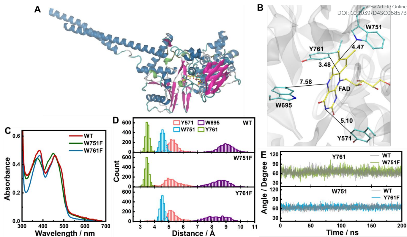
Fig. 1 (A) X-ray crystallographic structure of WT LSD1 (PDB entry: 2DW4). 51 (B) Electron-donating residues in the active site of WT LSD1 in the crystal structure (distances given in Å). (C) Steady-state absorption spectra of WT, W751F and Y761F LSD1. (D) Distributions of the edge-to-edge distances between FAD and close-by tyrosine and tryptophan residues in 200-ns MD simulations. (E) Dynamics of the angles between the ring planes of the isoalloxazine moiety of FAD and the indole or phenol moiety of Y761 or W751, during the MD simulations of WT, W751F and Y761F LSD1, as indicated.
